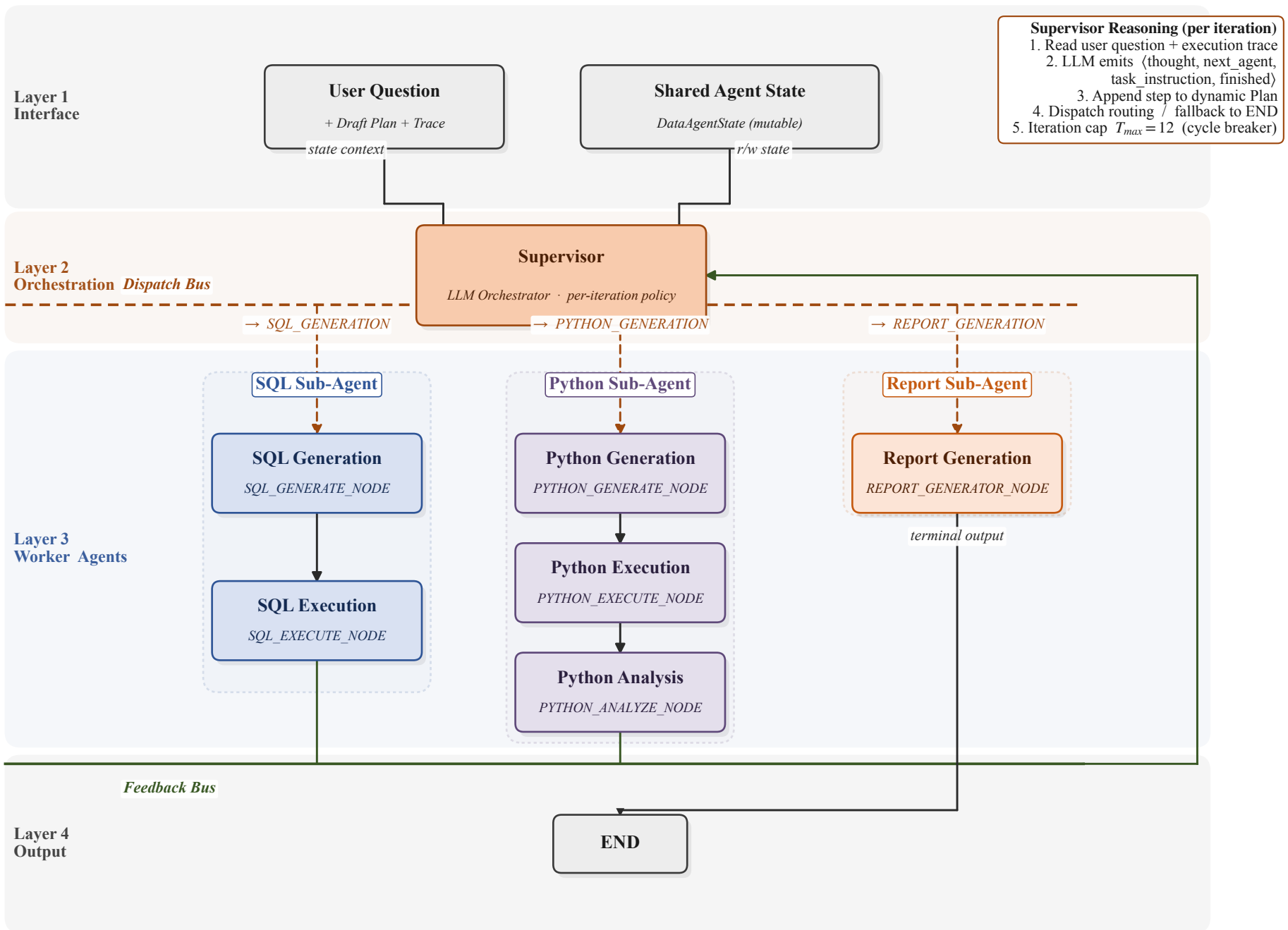
Fig. 2. Supervisor-Orchestrated Multi-Agent Architecture (Layered View)
