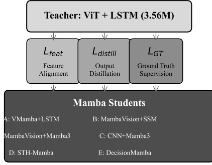
(A) Cross-Architecture Distillation Framework
