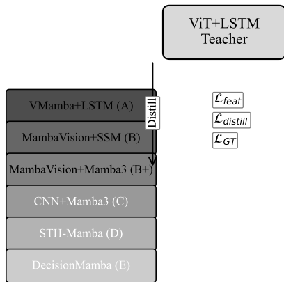
(A) Distillation Framework
