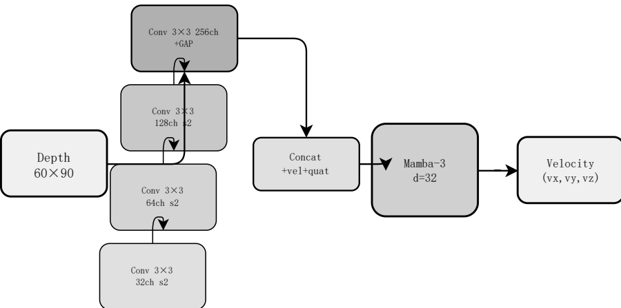
Branch C: CNN+Mamba-3 (2.41M params)
