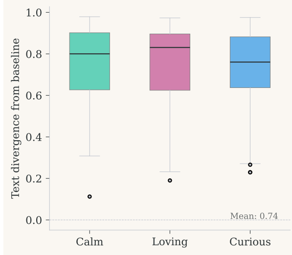
Figure 3: Text divergence from baseline by injection vector (normalized edit distance). All three vectors show 0.72–0.74 mean divergence at \alpha=0.1 ; however, a null-null control yields identical divergence (0.736), indicating this reflects stochastic decoding, not injection effects.
