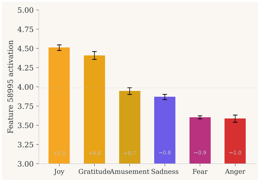
Figure 1: Feature 58995 mean activation by emotion category ( n=60 trials per emotion). Valence labels shown below each bar. Sadness ( -0.8 ) activates higher than fear ( -0.9 ) and anger ( -1.0 ), consistent with reflective depth rather than pure valence polarity.
