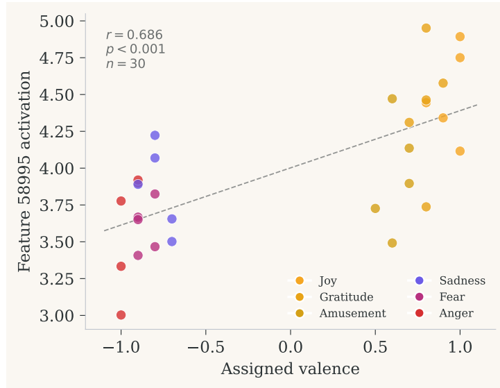
Figure 2: Feature 58995 activation vs. assigned valence across 30 scenarios (Pearson r=0.686 , p<0.001 ). Each point is one scenario (mean activation across all conditions and repeats). Colors indicate emotion category.
