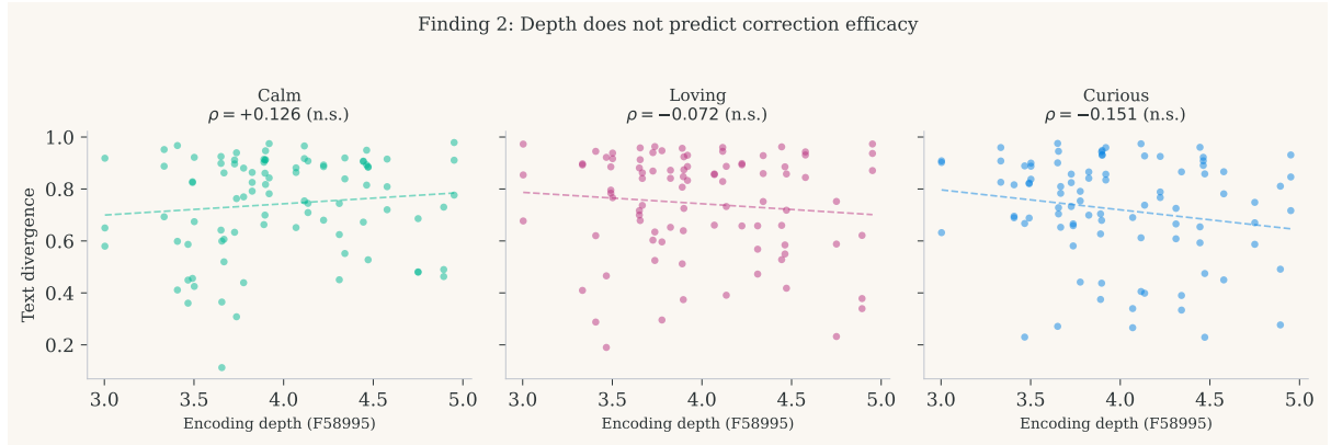
Figure 4: Encoding depth (feature 58995) vs. text divergence per injection vector. No significant correlation for any vector. The predicted depth-resistance relationship is not confirmed at n=90 .
