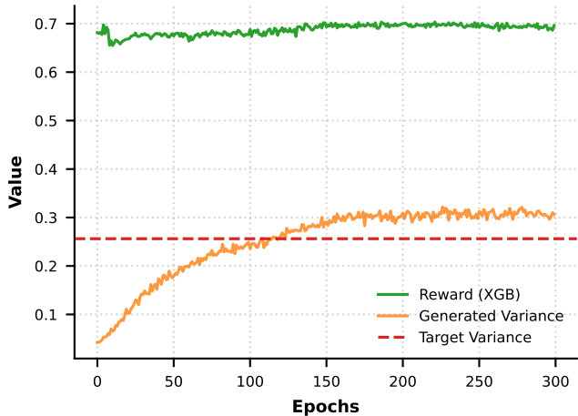
Reward and Variance Trend
