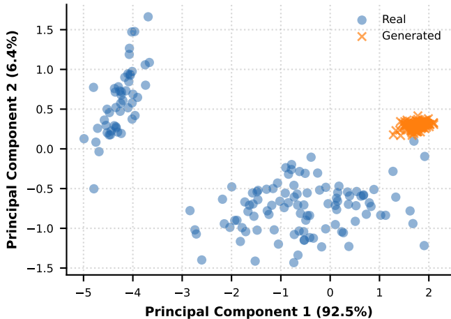
PCA: Distribution Overlap
