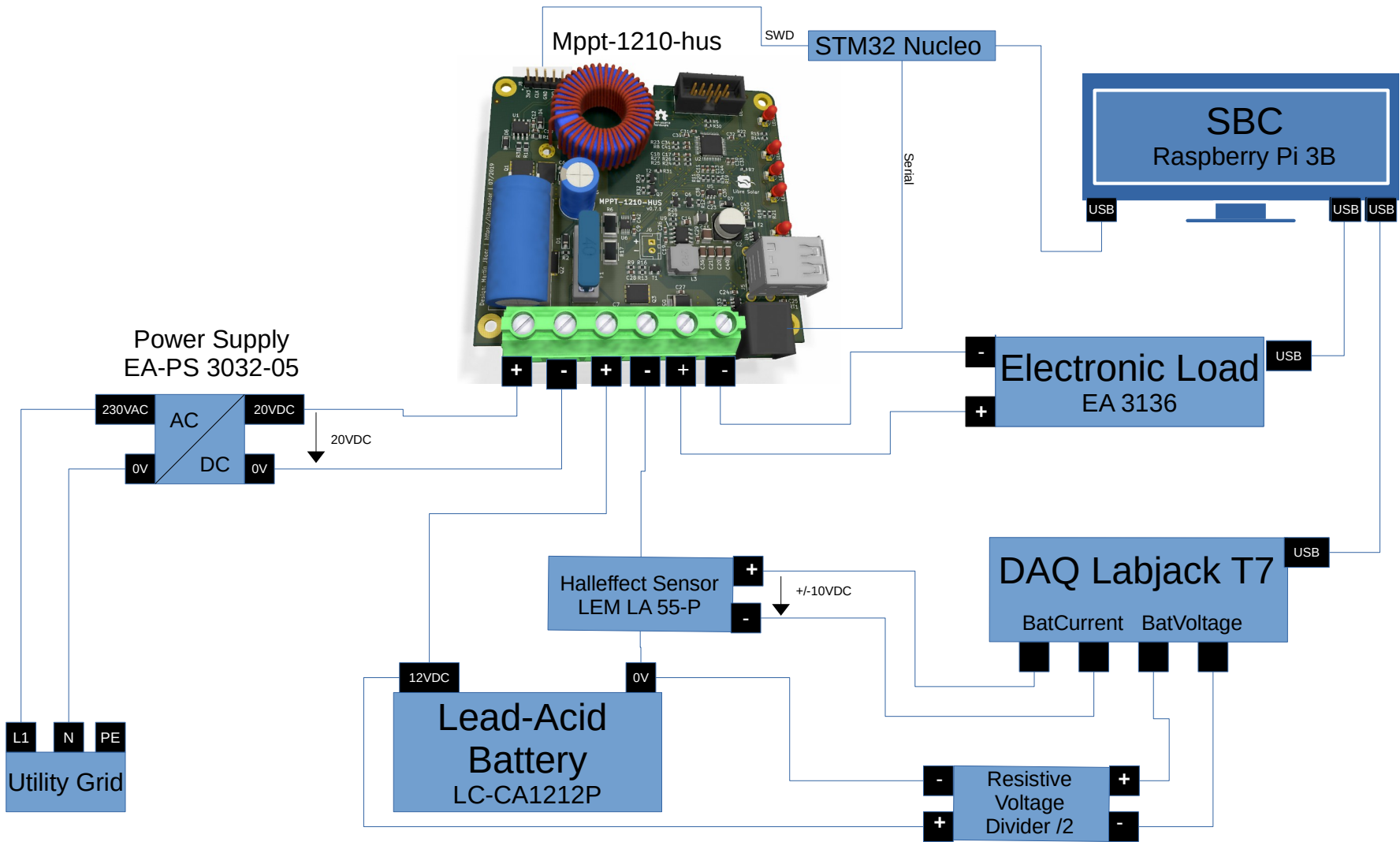
Hardware setup for validation of SOC-Algorithm by Emile Schons 22.06.21
