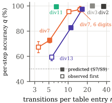
(b) per-step accuracy q vs. m
