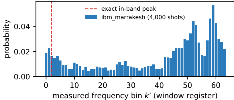
6-qubit windowed circuit, 138 CZ: device histogram
