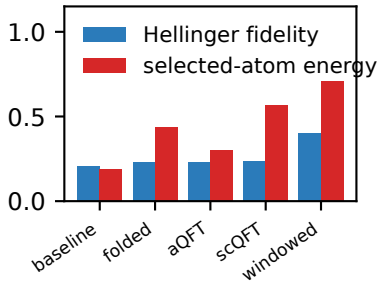
Heron noise model, mean of 12 cases
