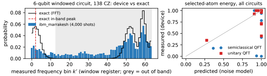
Figure 3: Left: device histogram of a 6-qubit windowed selection circuit on ibm_marrakesh against the exact distribution; grey bins are out of band (mirror frequencies) and are masked before selection. Right: selected-atom energy predicted by the calibrated noise model against the value measured on the device, all circuits.
