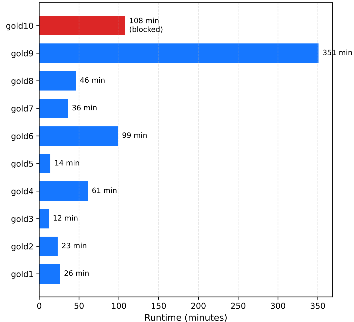
Runtime Duration
