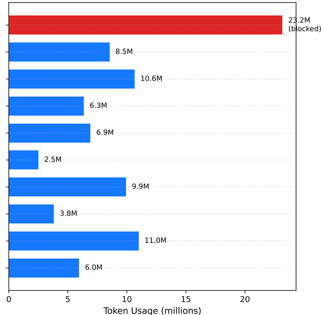
Token Consumption
