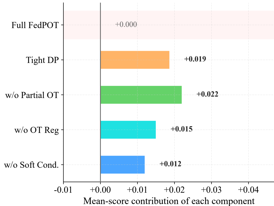
(b) Component Effect
