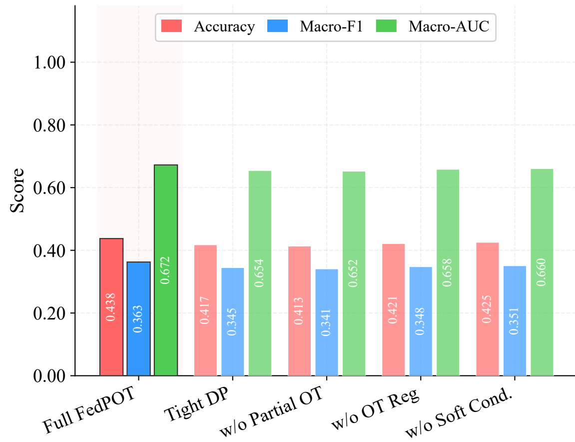
(a) Ablation Variant Performance
