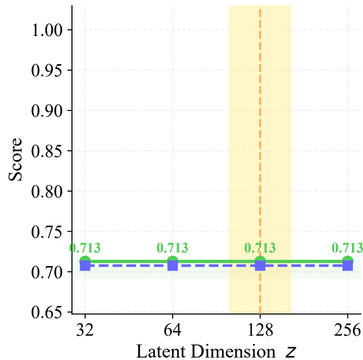
(c) Sensitivity to Latent Dimension z
