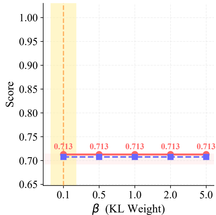
(a) Sensitivity to \beta (KL Weight)
