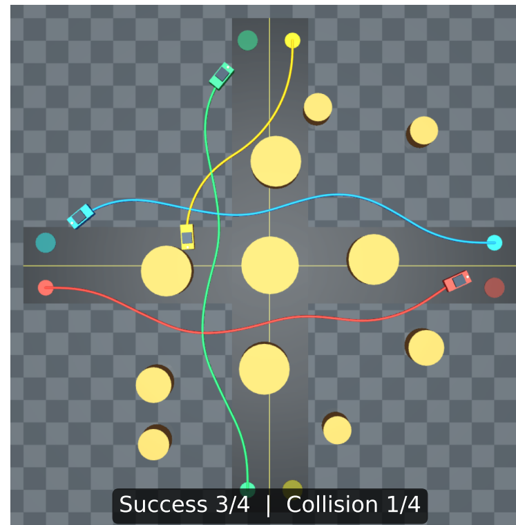
Stochastic MPC
