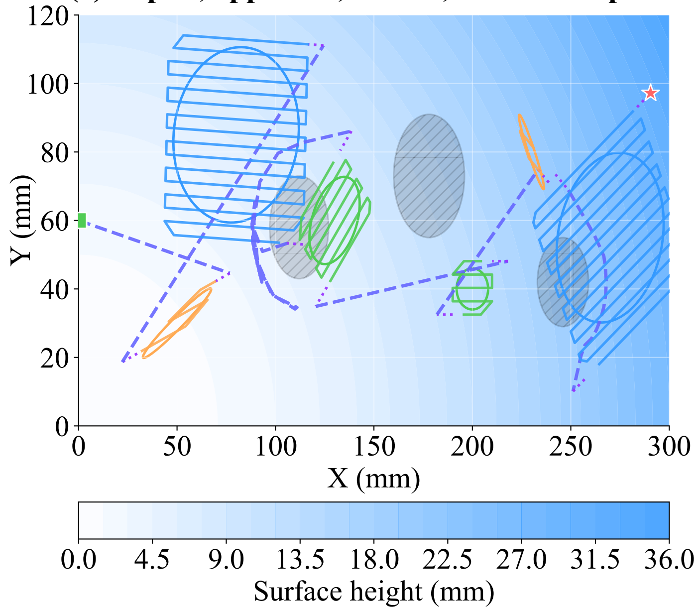
(a) Repair, approach, retract, and transit paths (b) Tool-height distribution along the trajectory
