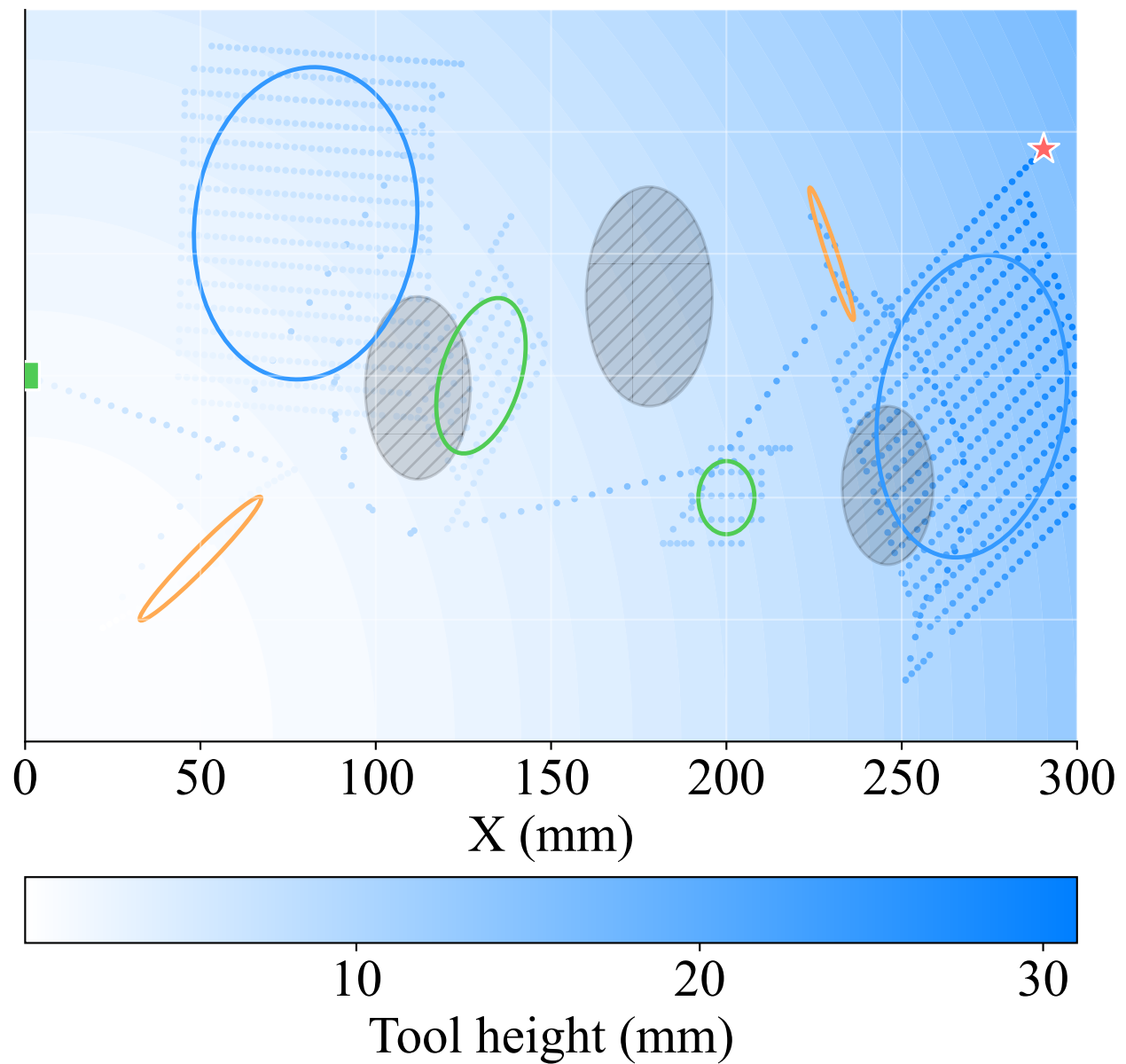
(a) Repair, approach, retract, and transit paths (b) Tool-height distribution along the trajectory
