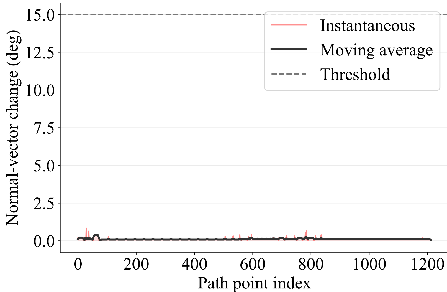
(a) Tool-normal change along the full path
