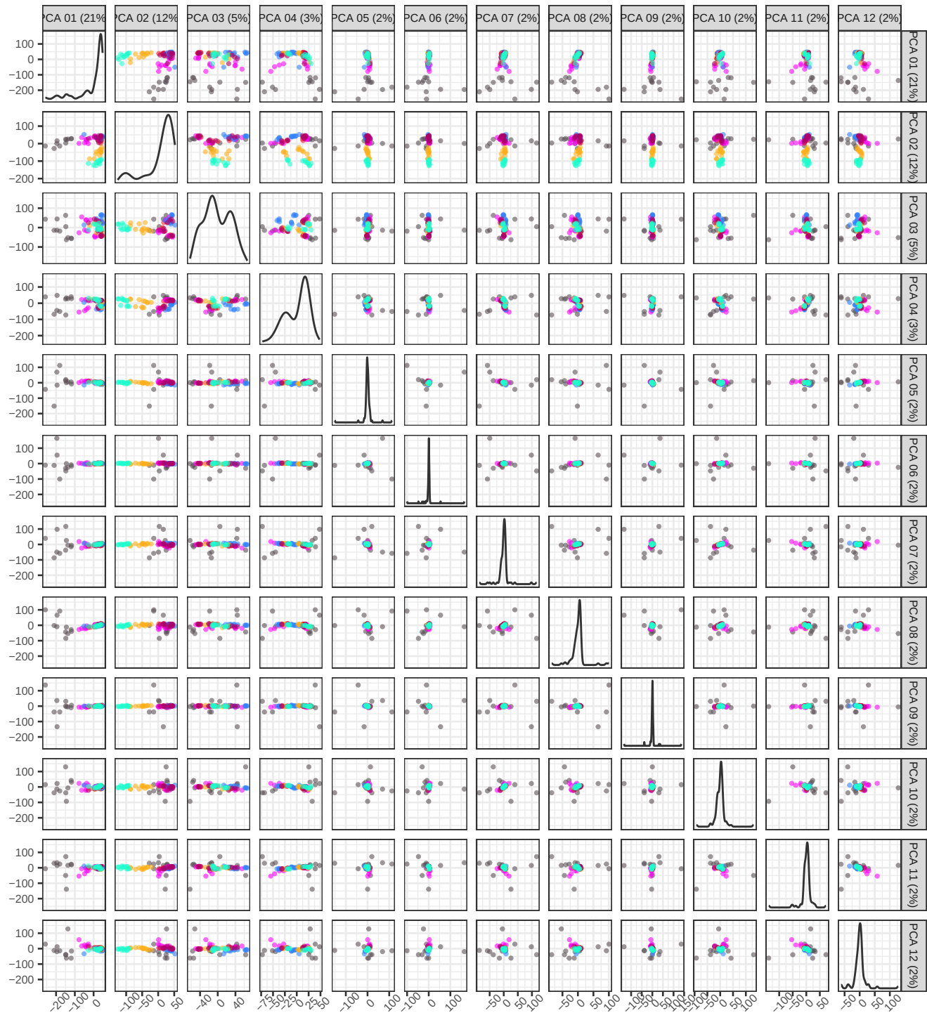
PCA of pseudobulk data with BS k=9
