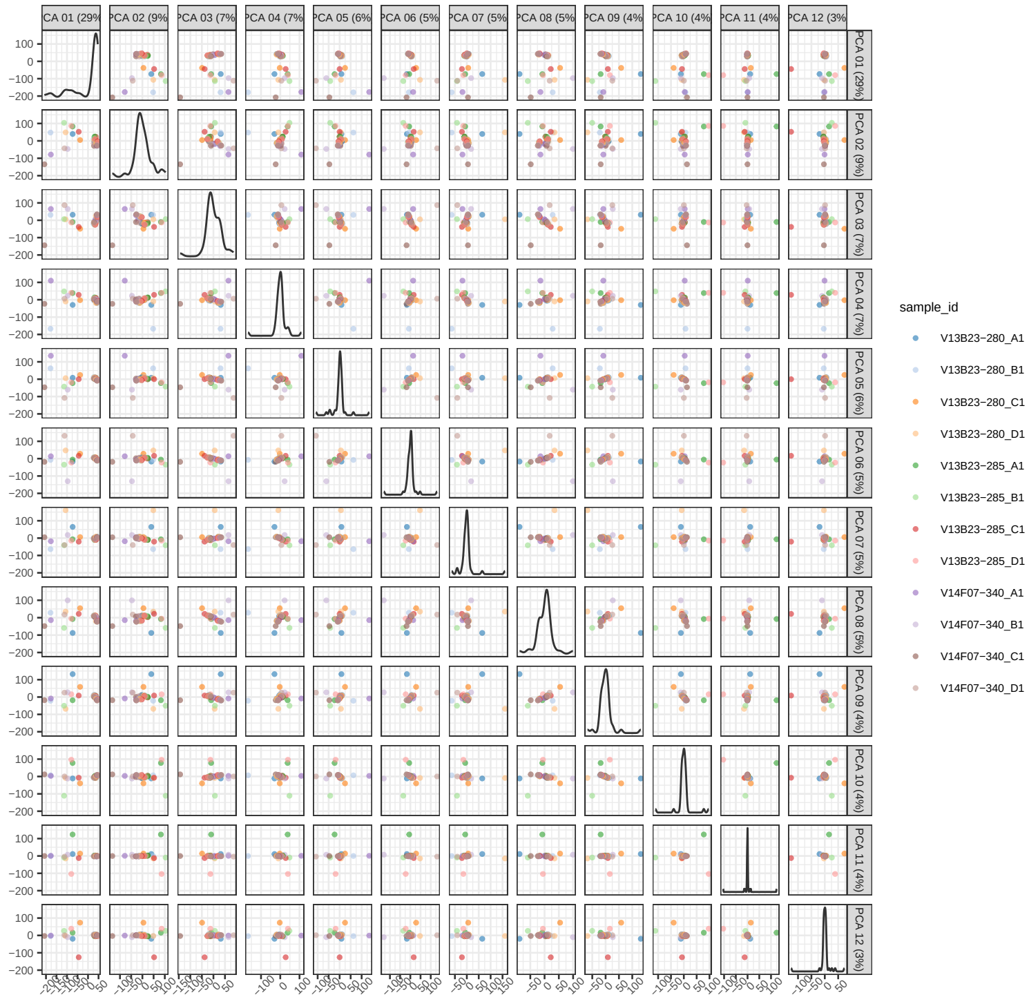
PCA of pseudobulk data with BS k=4
