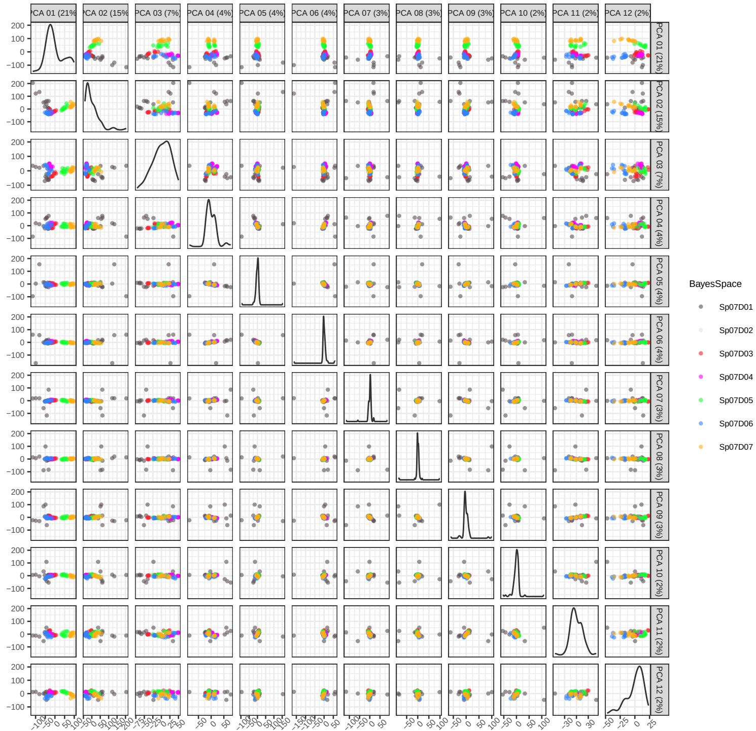
PCA of pseudobulk data with BS k=7
