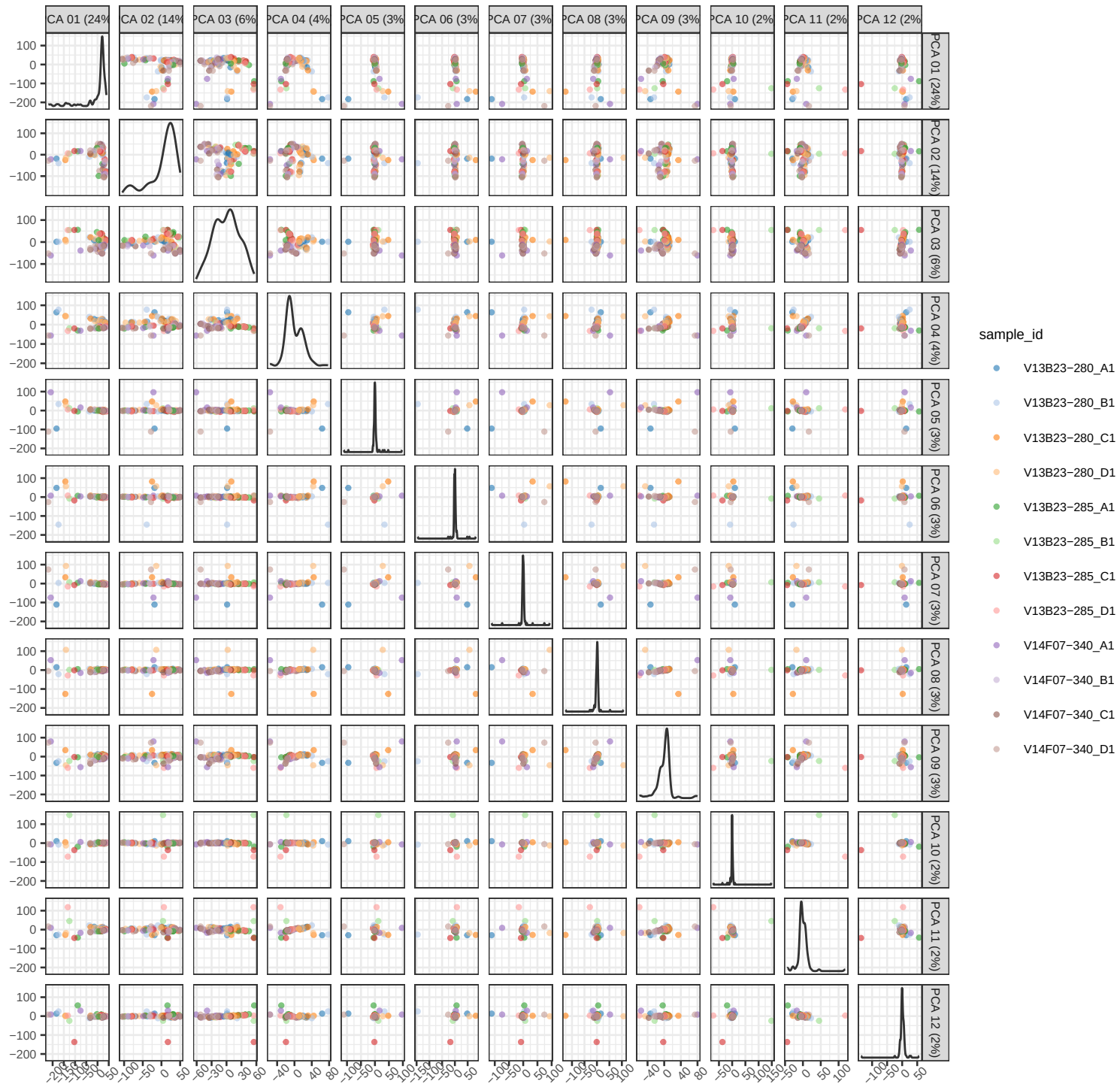
PCA of pseudobulk data with BS k=10
