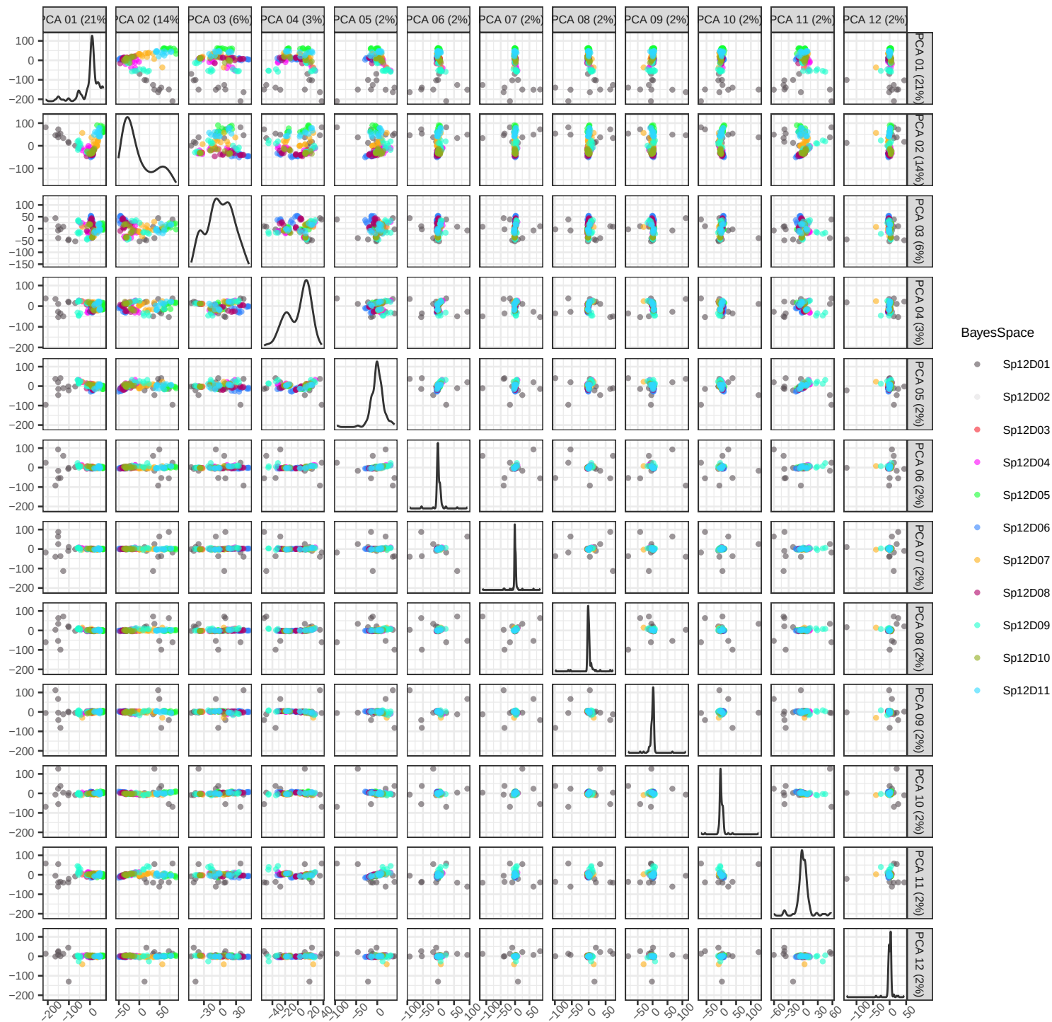
PCA of pseudobulk data with BS k=12
