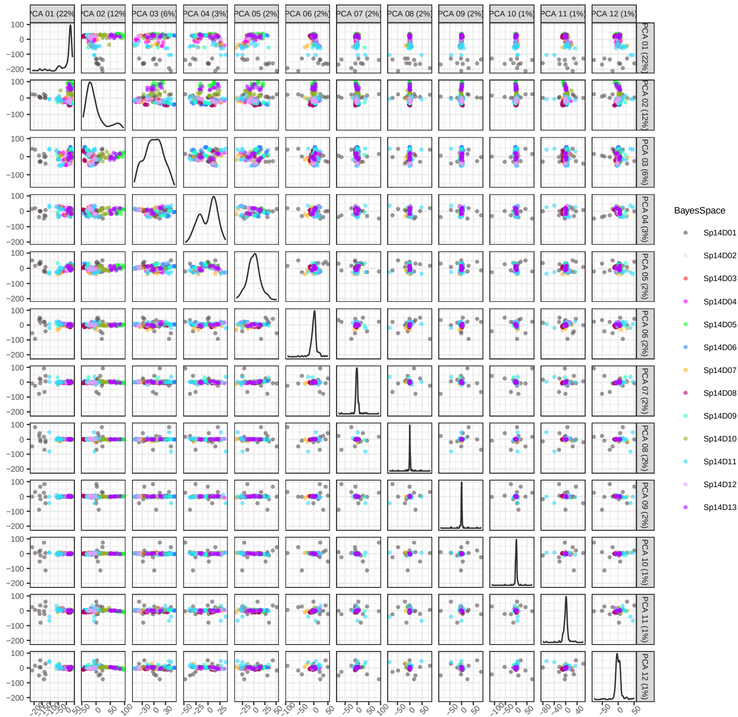
PCA of pseudobulk data with BS k=14
