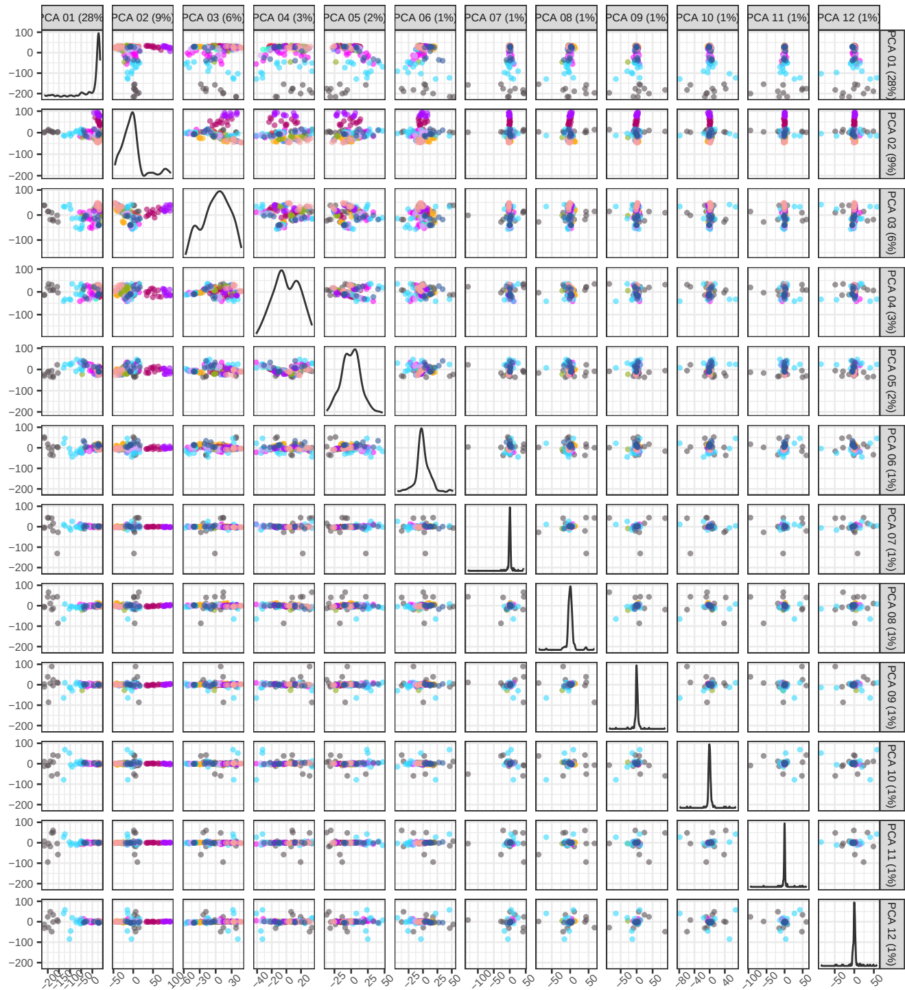
PCA of pseudobulk data with BS k=15
