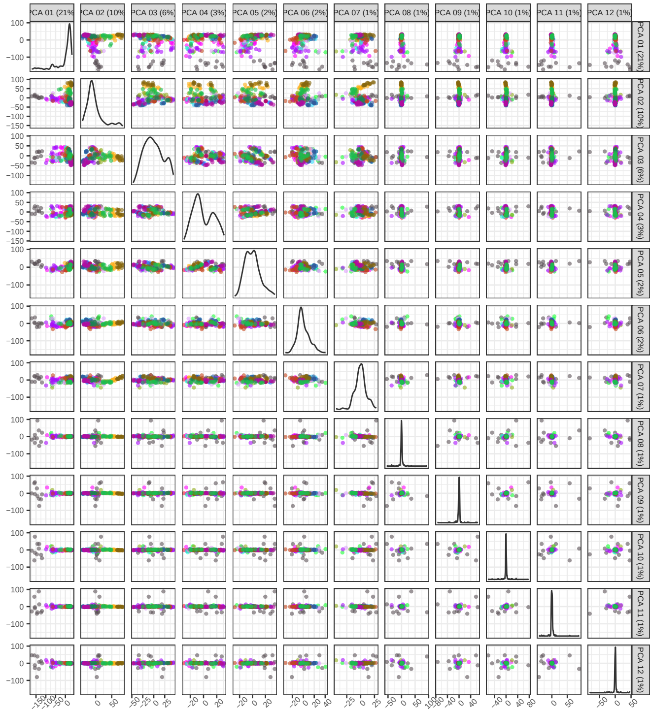
PCA of pseudobulk data with BS k=21
