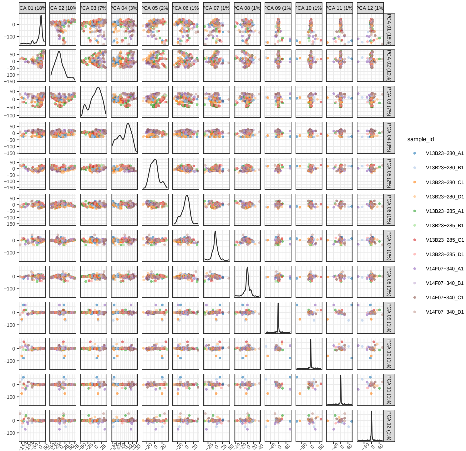
PCA of pseudobulk data with BS k=24
