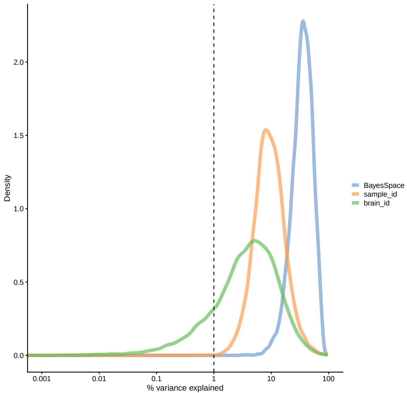
PCA of pseudobulk data with BS k=14
