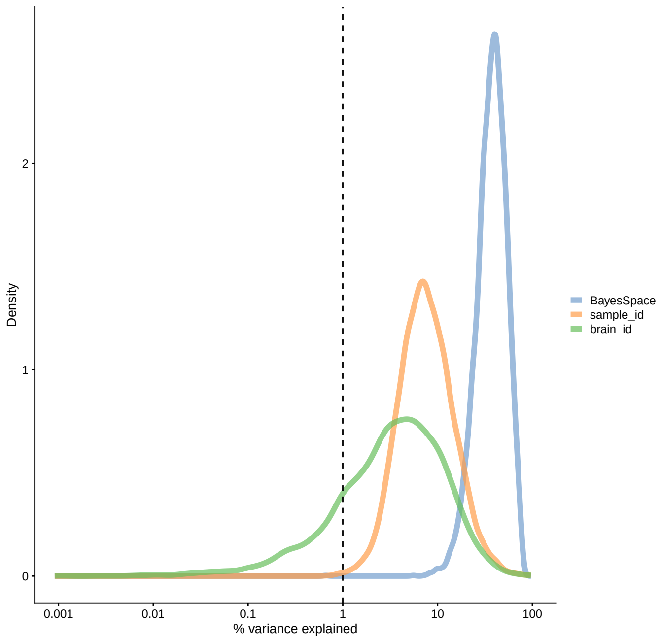
PCA of pseudobulk data with BS k=20
