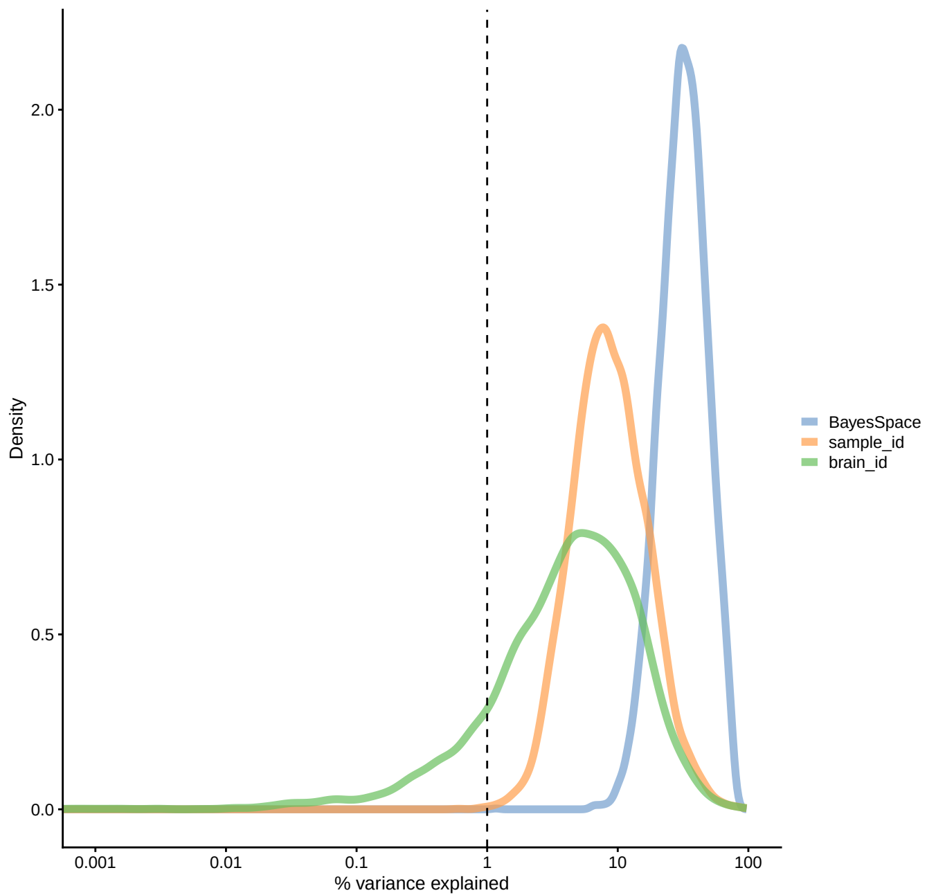
PCA of pseudobulk data with BS k=23
