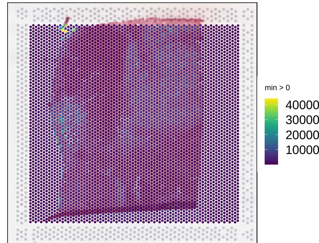
V13B23-285_C1 sum_umi
