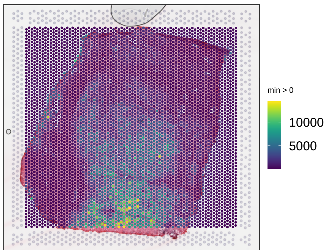
V13B23-285_A1 sum_umi
