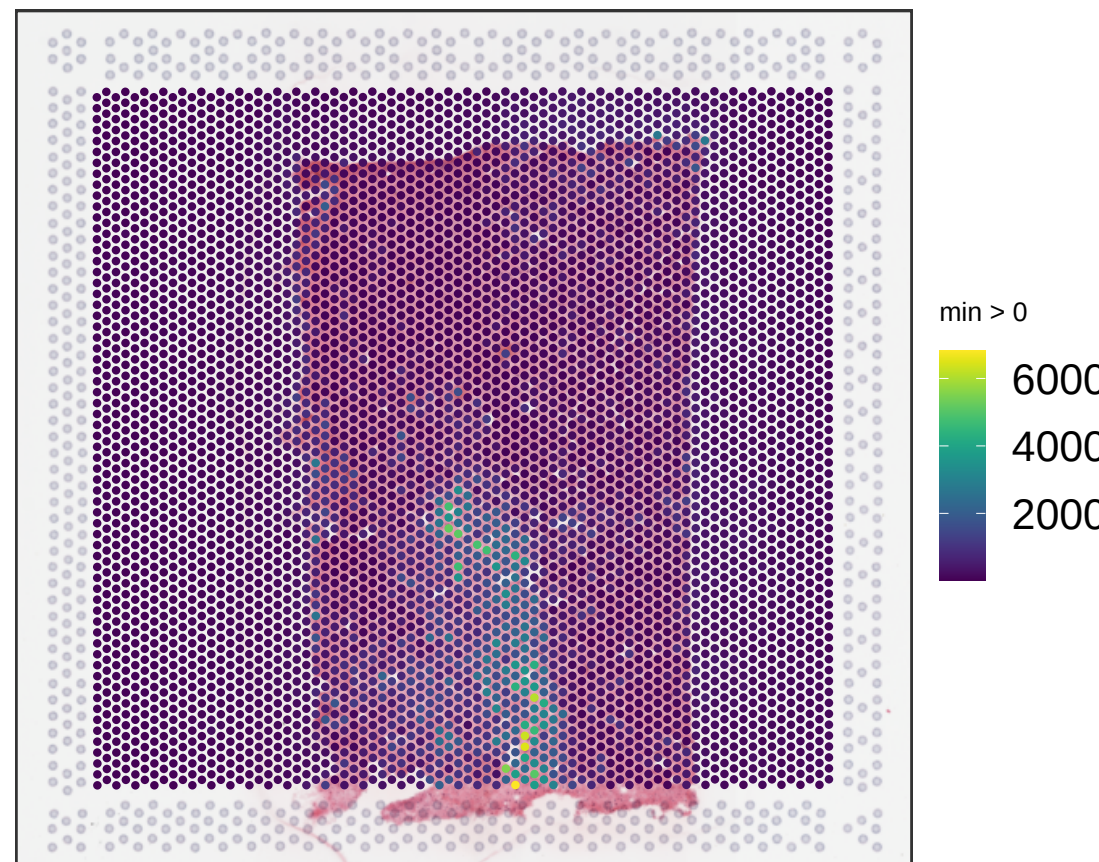
V13B23-281_B1 sum_umi
