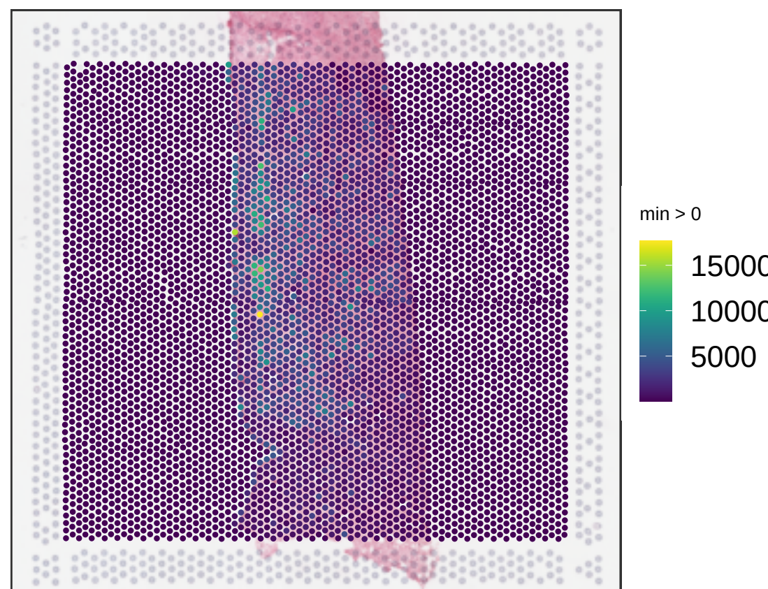
V14F07-340_B1 sum_umi
