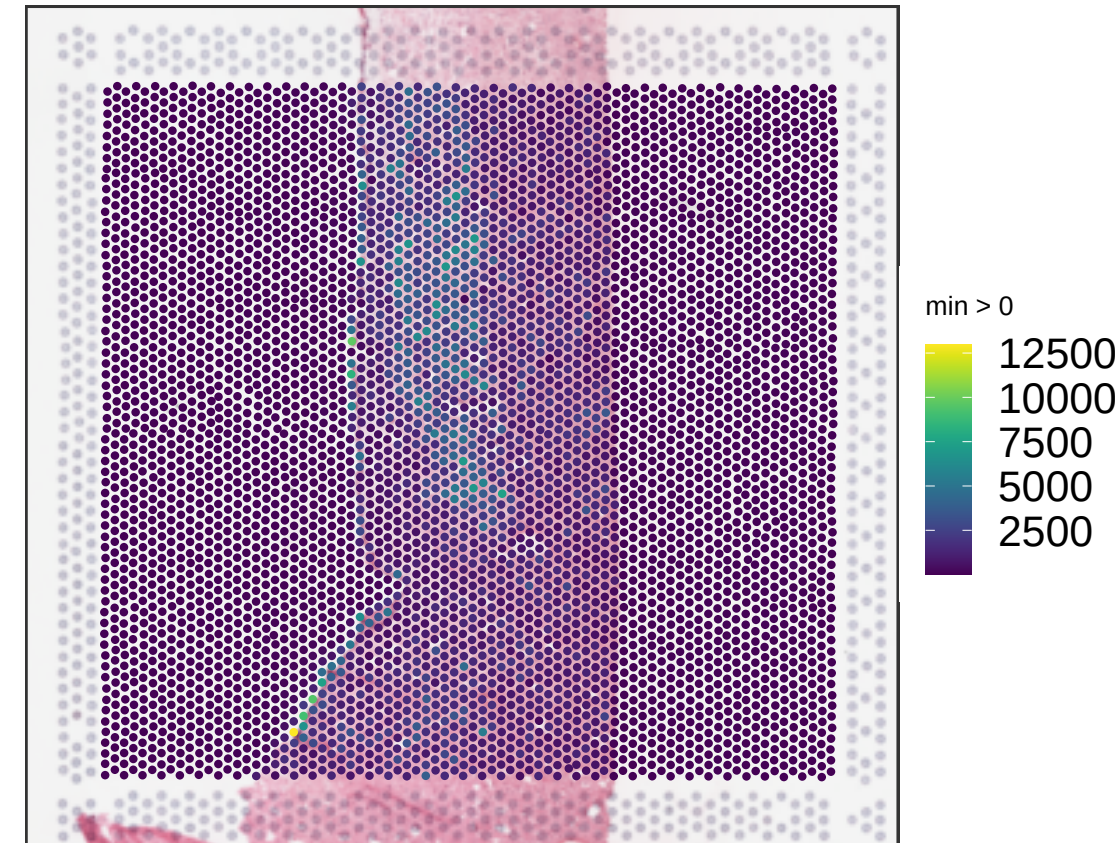
V14F07-340_C1 sum_umi
