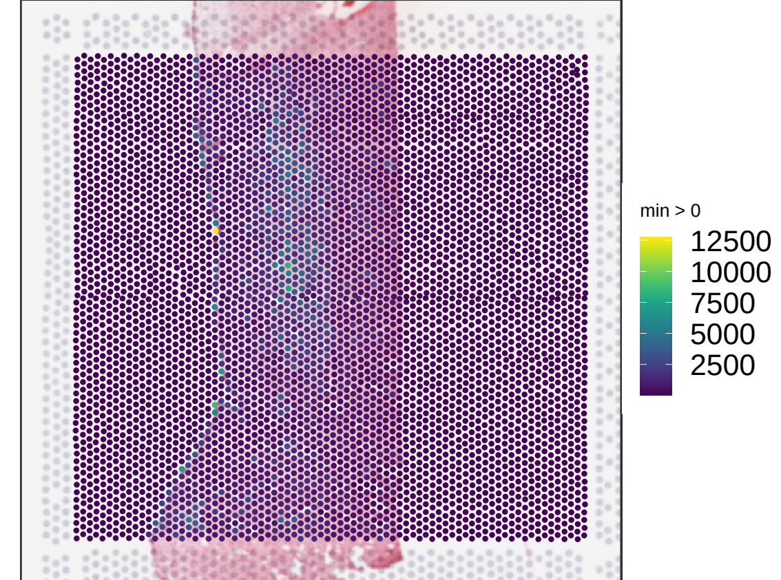
V14F07-340_D1 sum_umi
