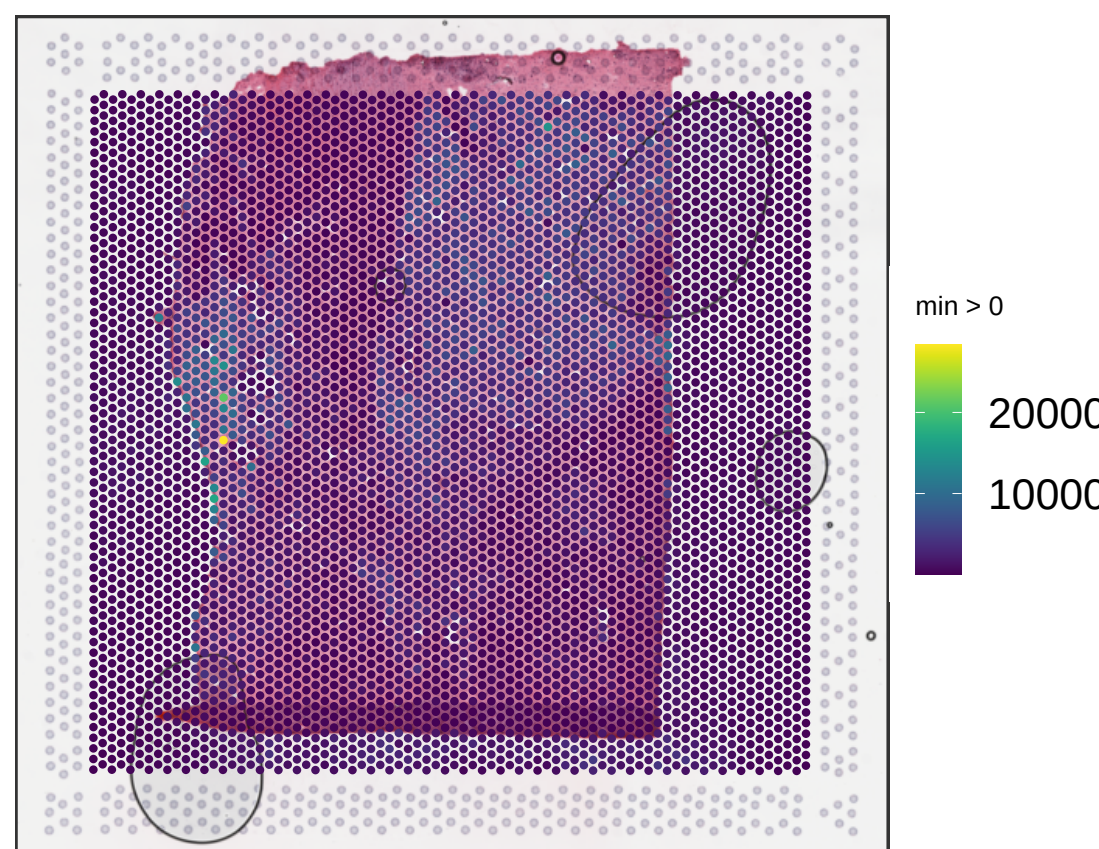
V13B23-285_B1 sum_umi
