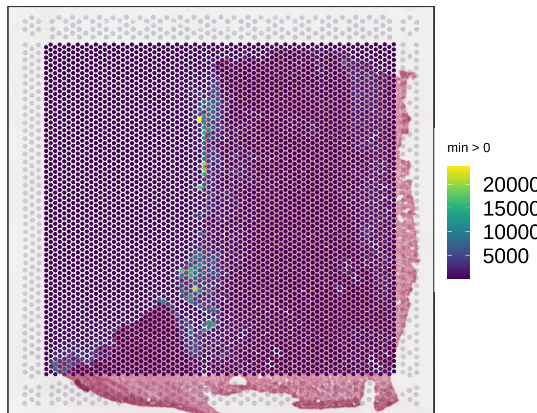
V13B23-280_B1 sum_umi
