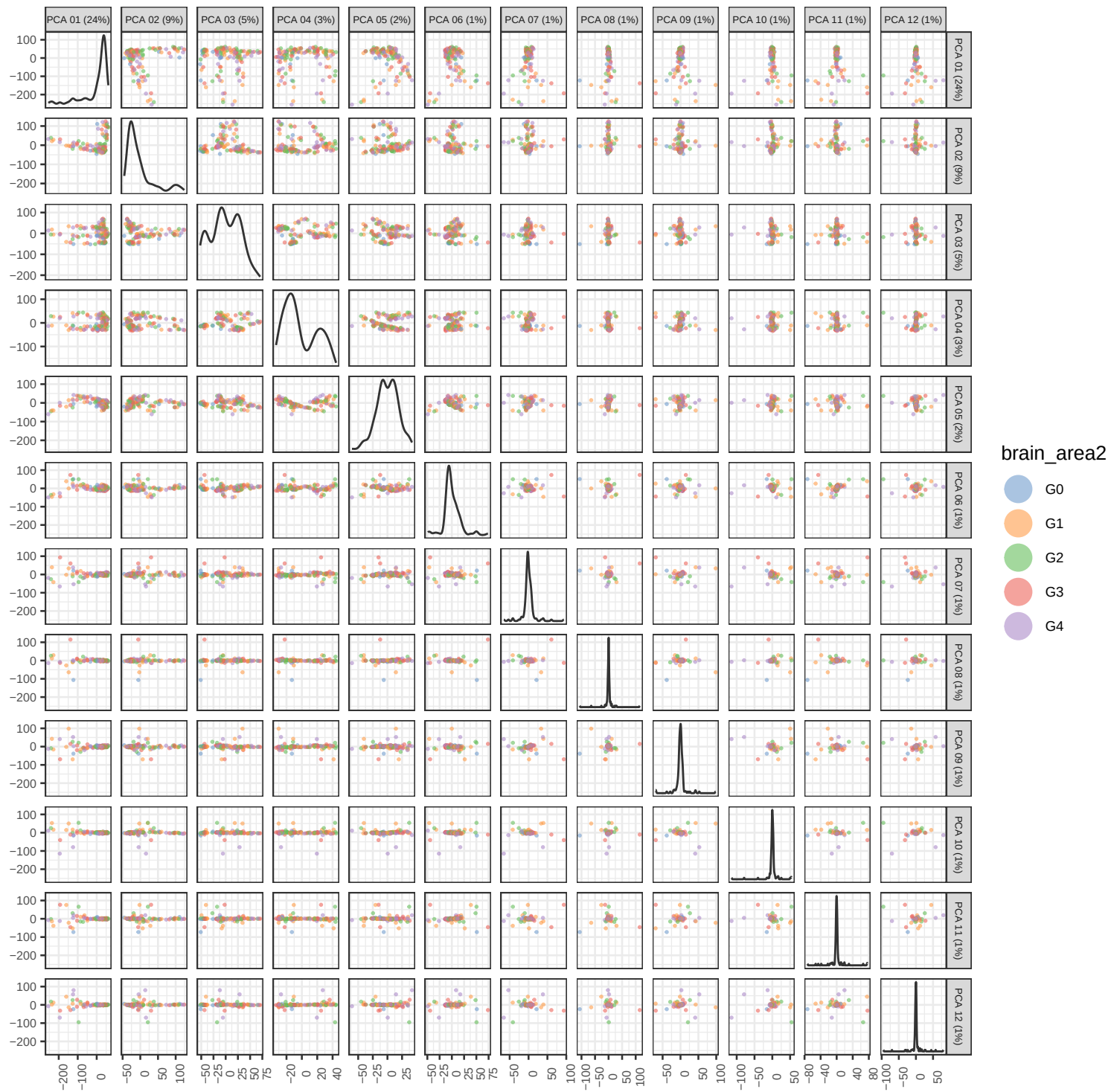
PCA of pseudobulk data with BS k=13
