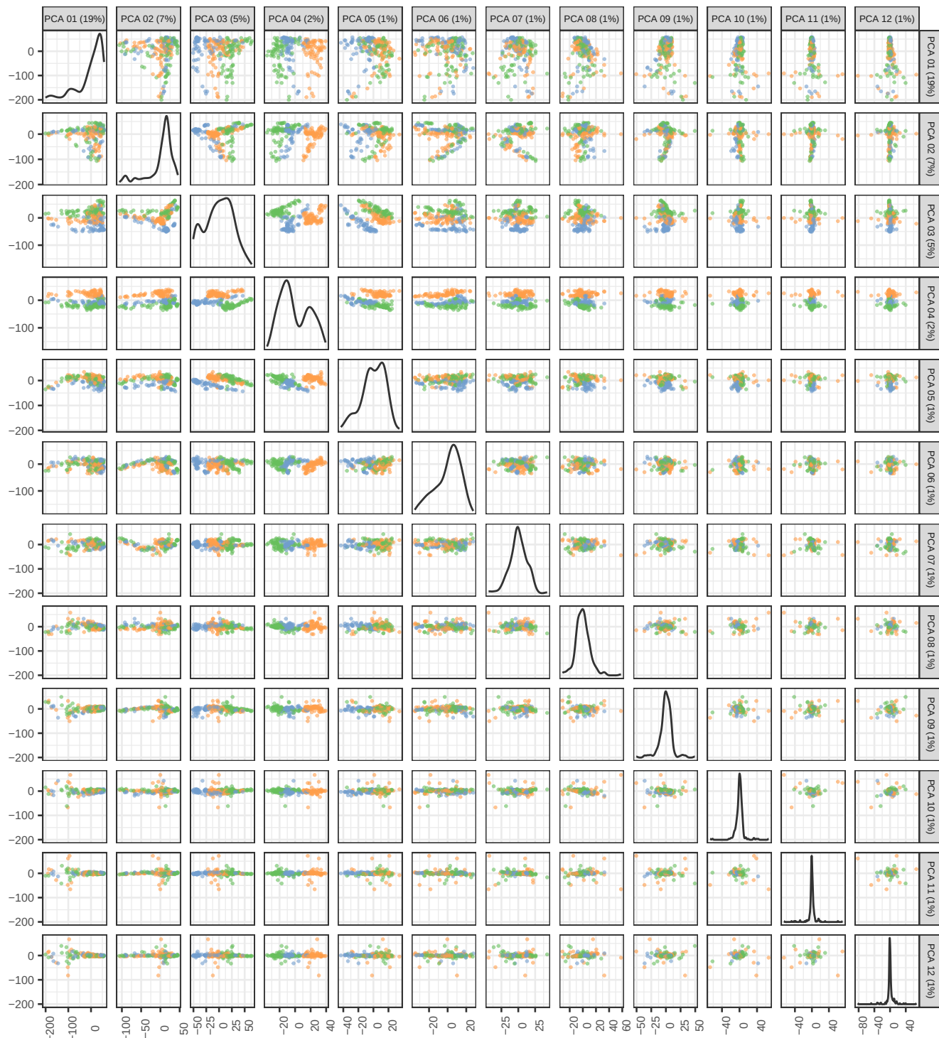
PCA of pseudobulk data with BS k=21
