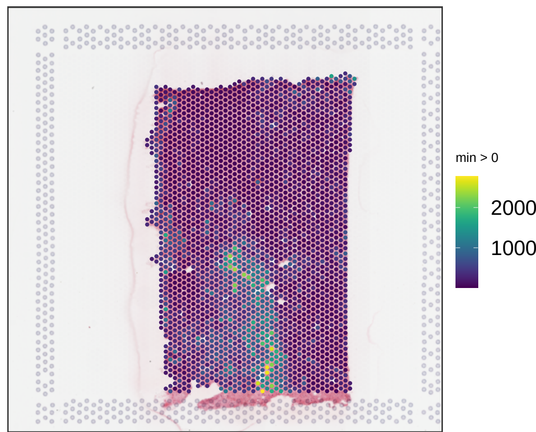
V13B23-281_B1 sum_gene
