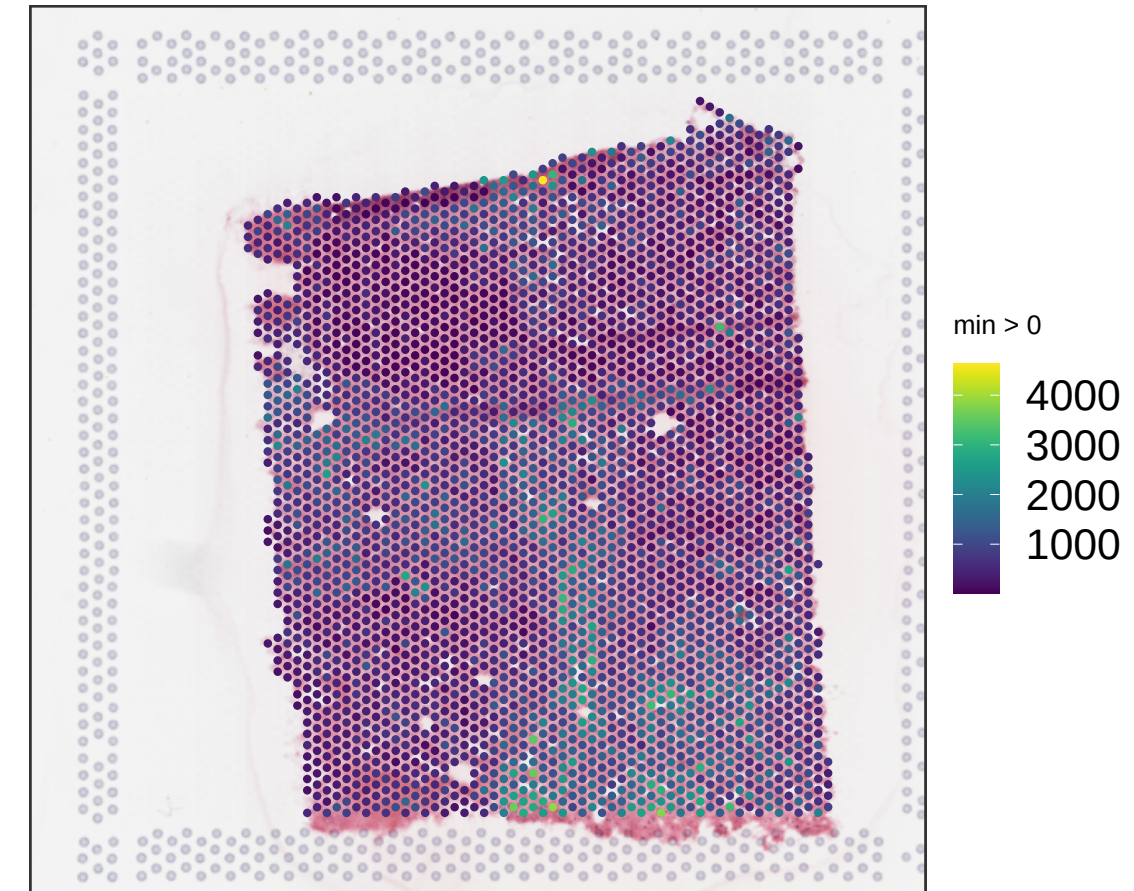
V13B23-281_D1 sum_gene
