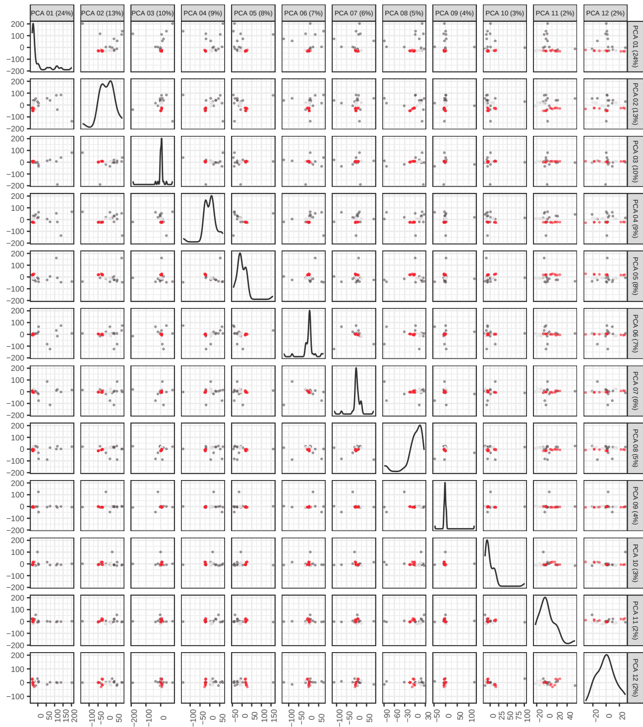
PCA of pseudobulk data with BS k=3
