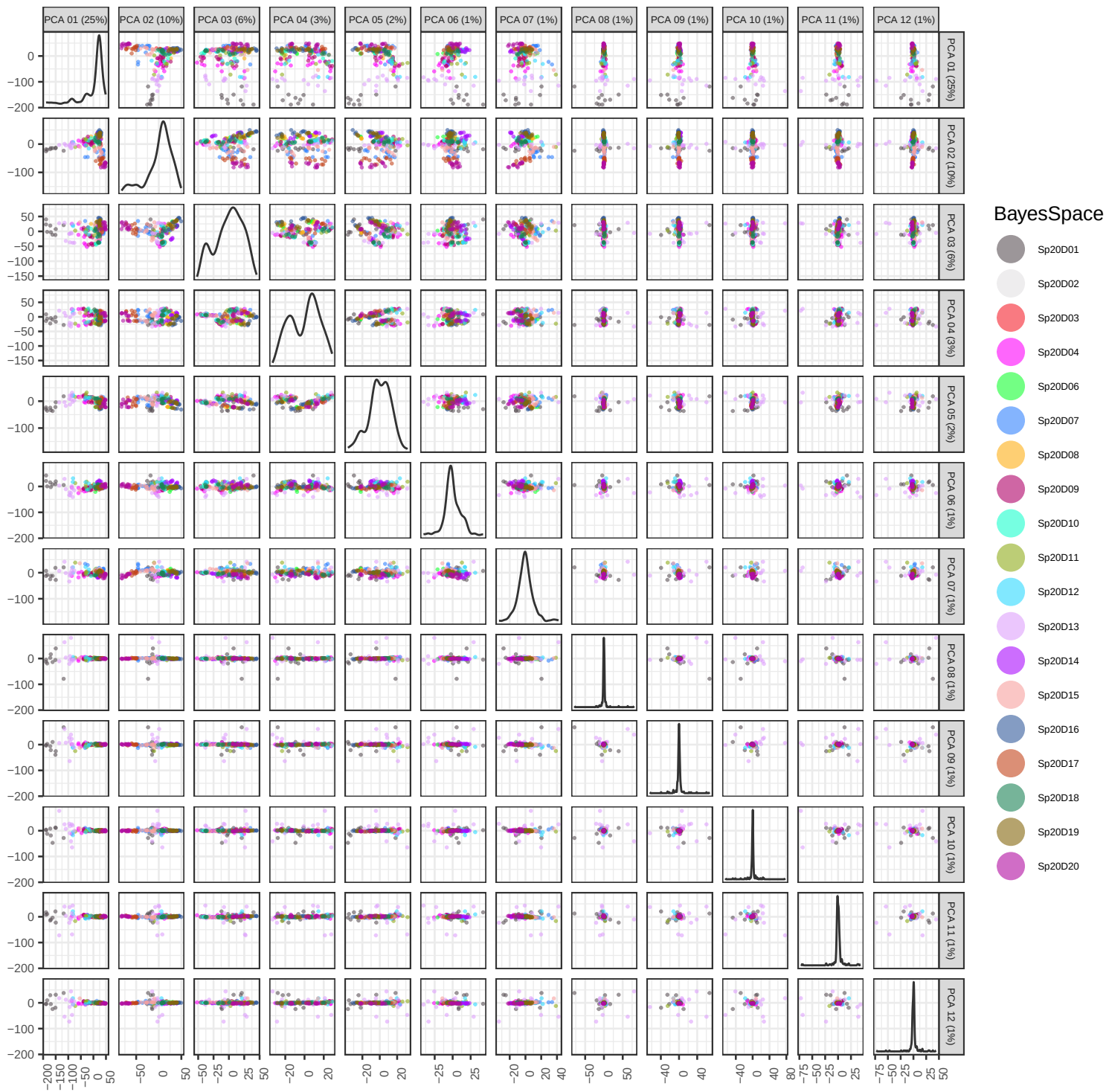
PCA of pseudobulk data with BS k=20
