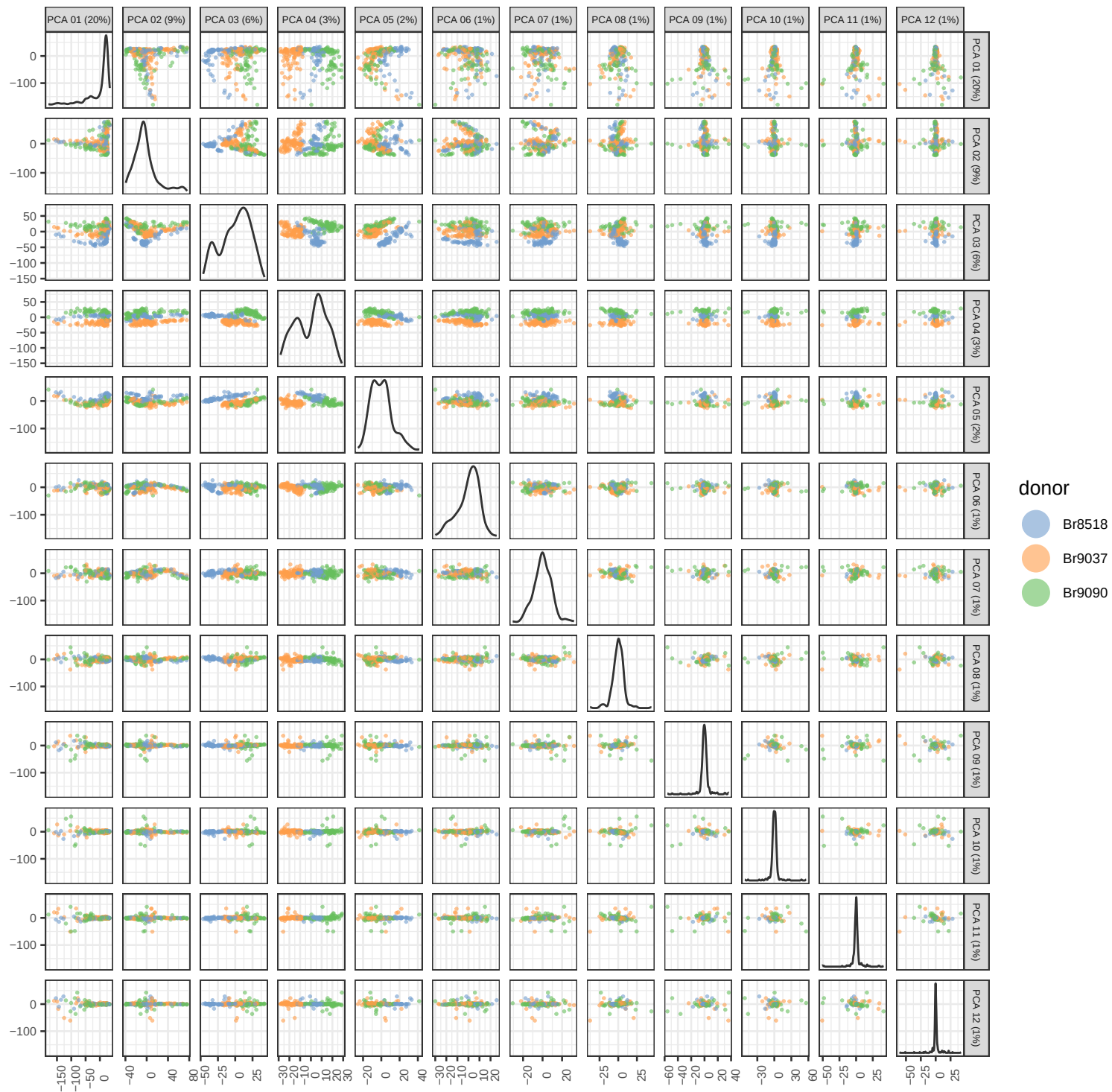
PCA of pseudobulk data with BS k=28
