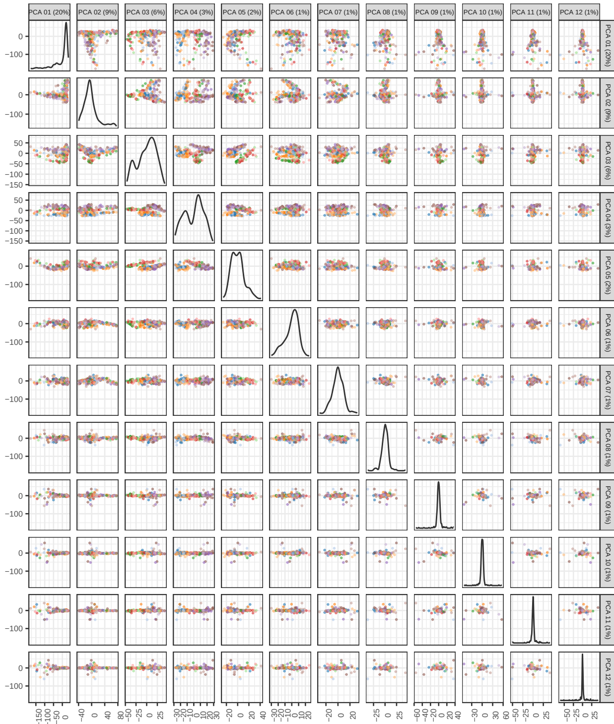
PCA of pseudobulk data with BS k=28
