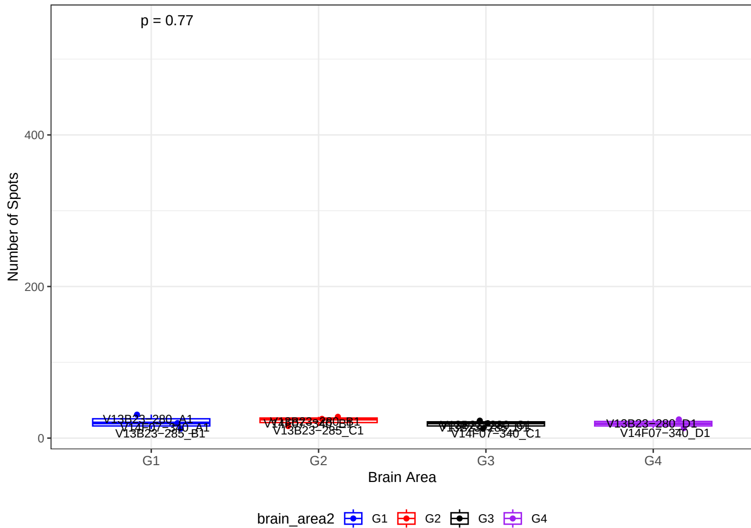
BayesSpace Domain: Sp28D25
