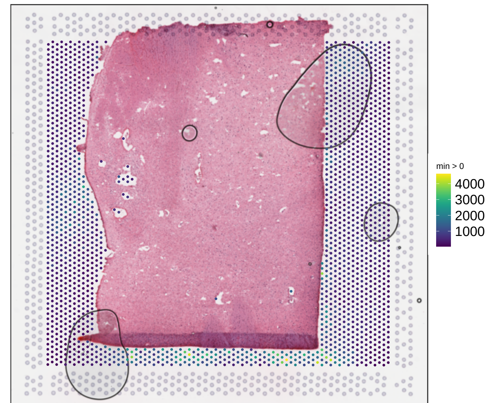
V13B23-285_B1 sum_umi
