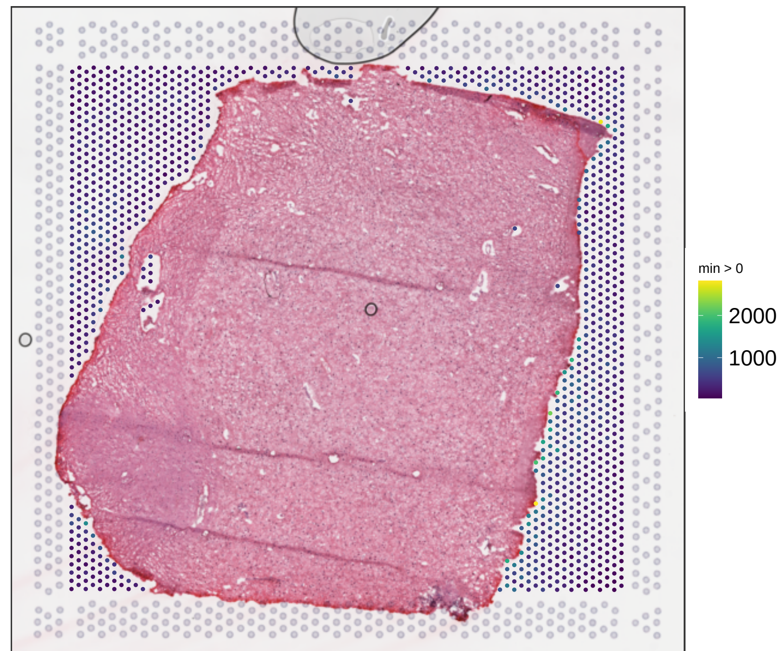
V13B23-285_A1 sum_umi
