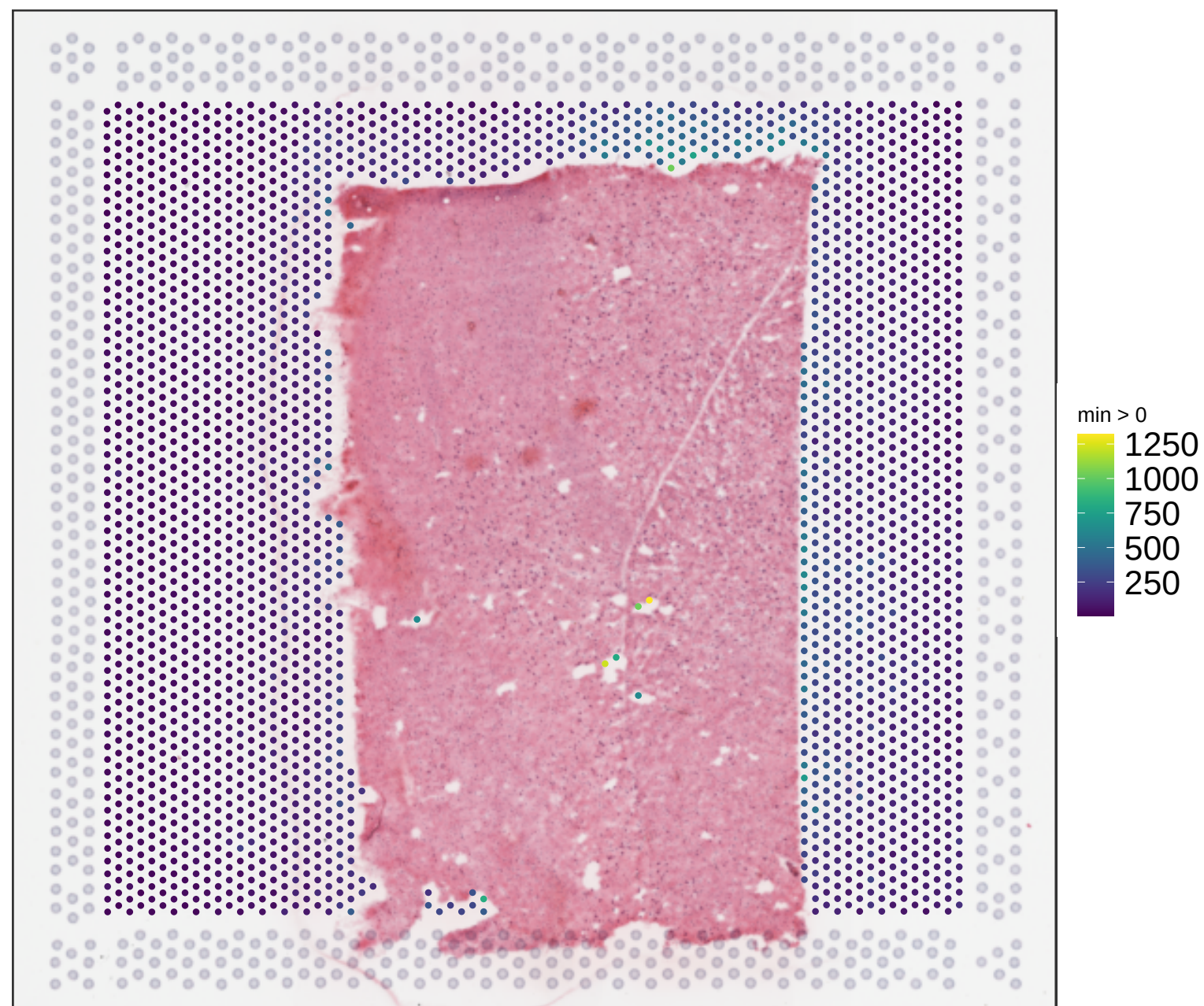
V13B23-281_B1 sum_umi
