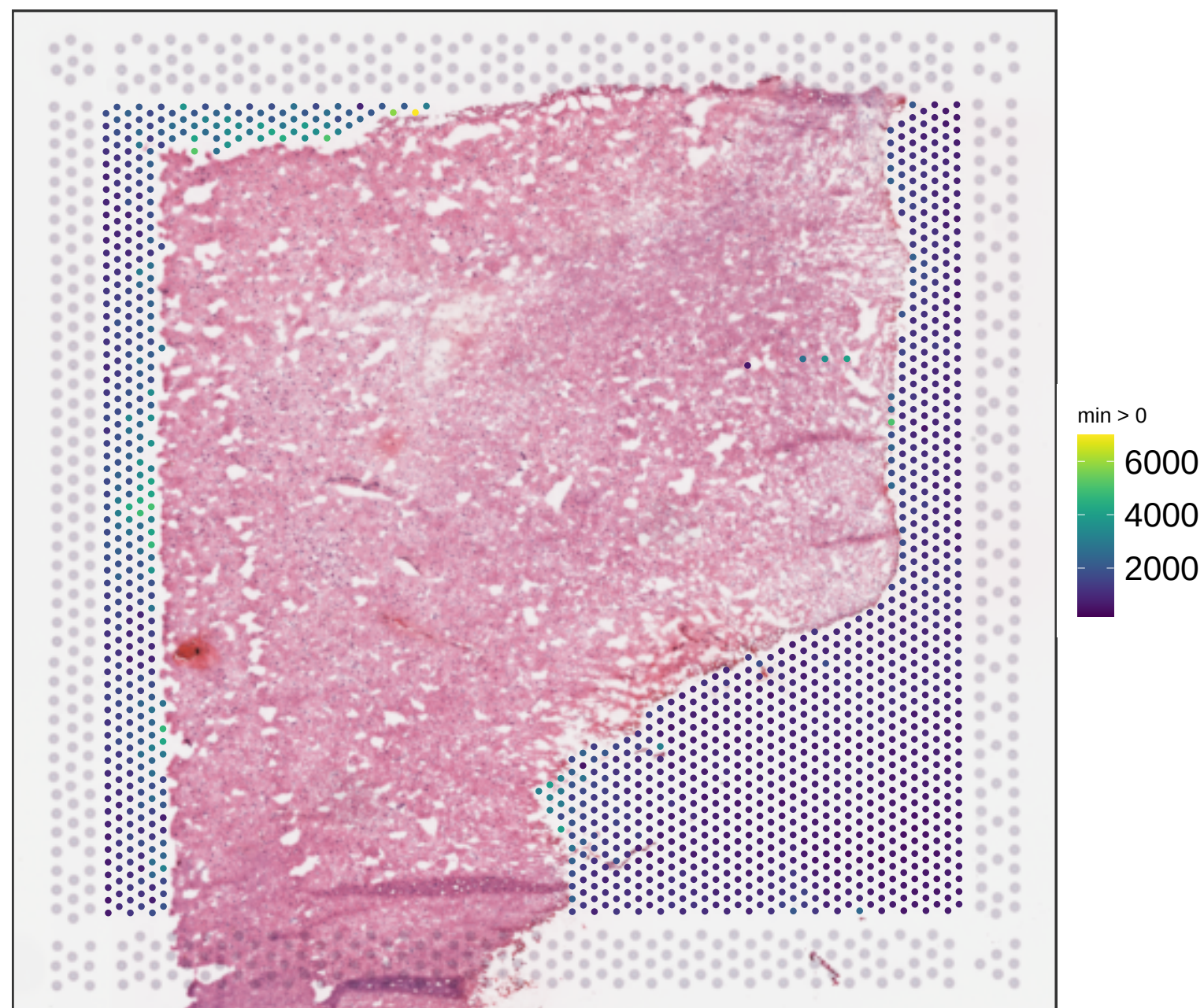
V12D07-075_C1 sum_umi
