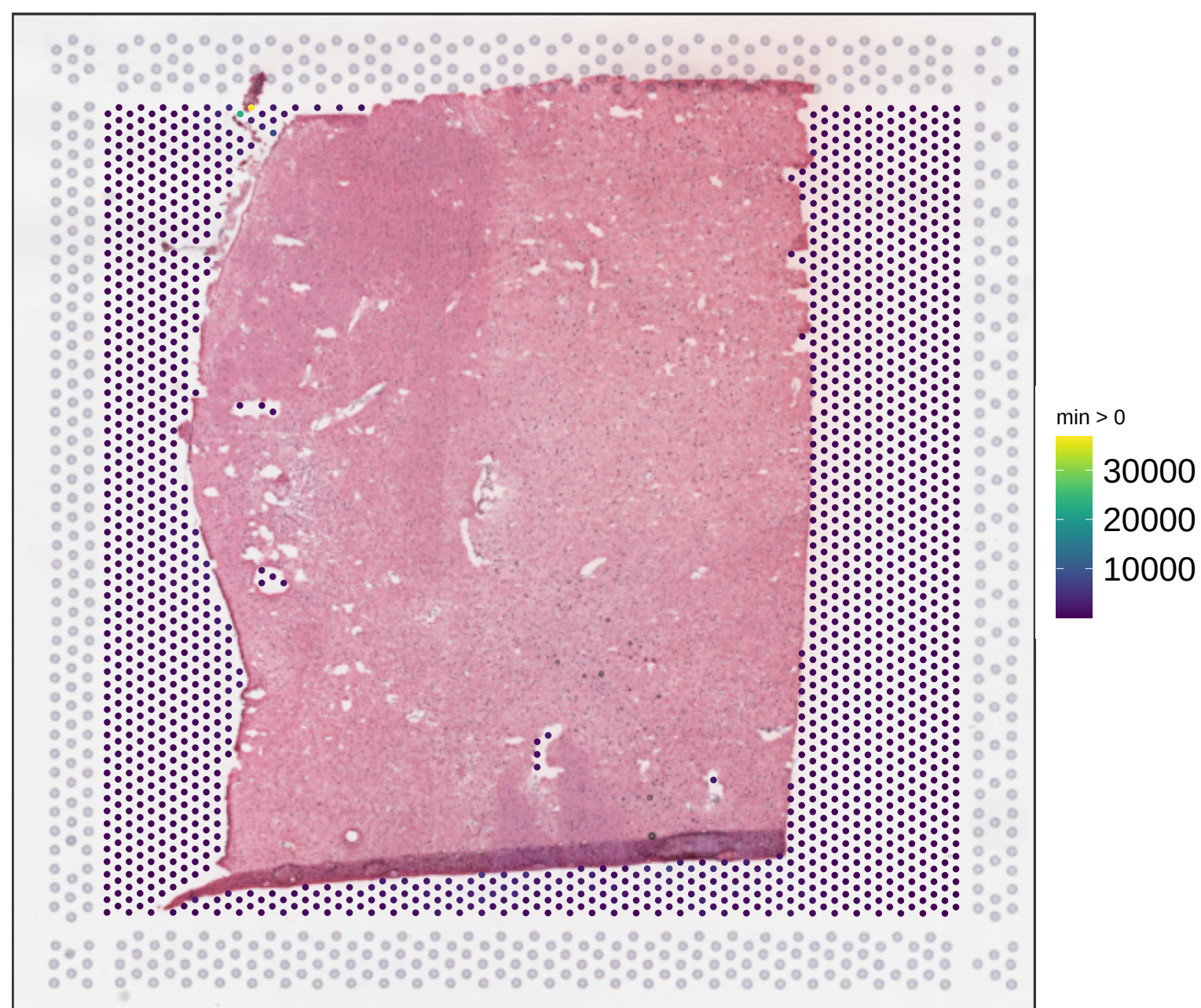
V13B23-285_C1 sum_umi
