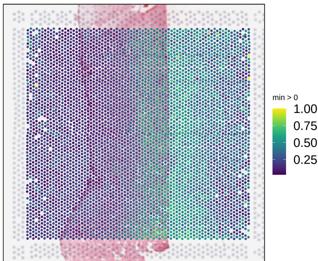
V14F07-340_D1 expr_chrm_ratio
