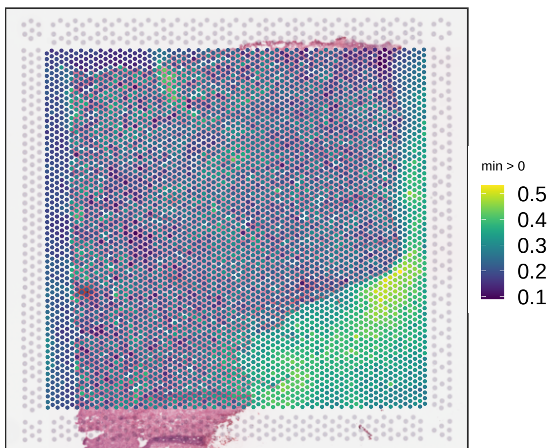
V12D07-075_C1 expr_chrm_ratio
