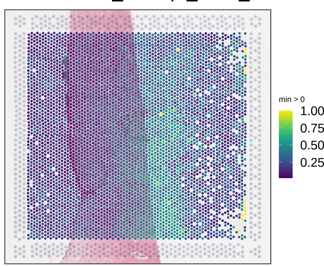
V14F07-340_A1 expr_chrm_ratio
