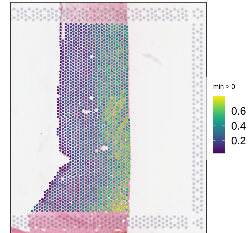
V14F07-340_C1 expr_chrm_ratio
