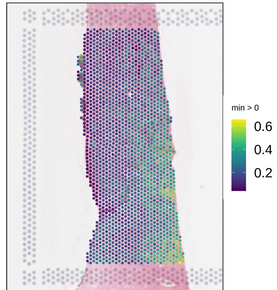
V14F07-340_A1 expr_chrm_ratio
