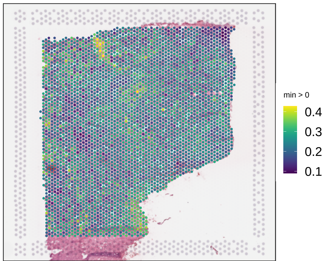
V12D07-075_C1 expr_chrm_ratio
