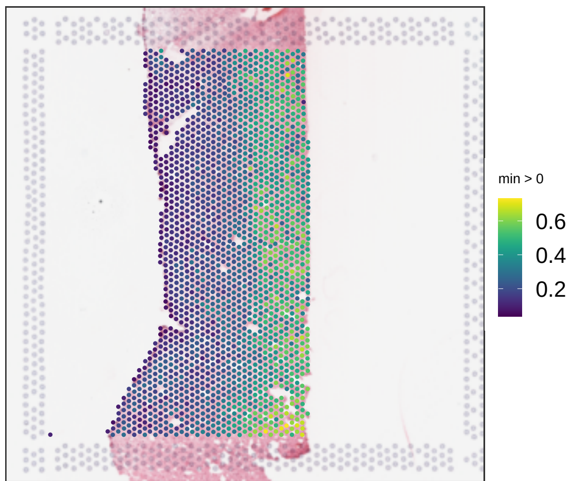
V14F07-340_D1 expr_chrm_ratio
