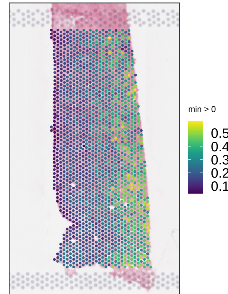
V14F07-340_B1 expr_chrm_ratio
