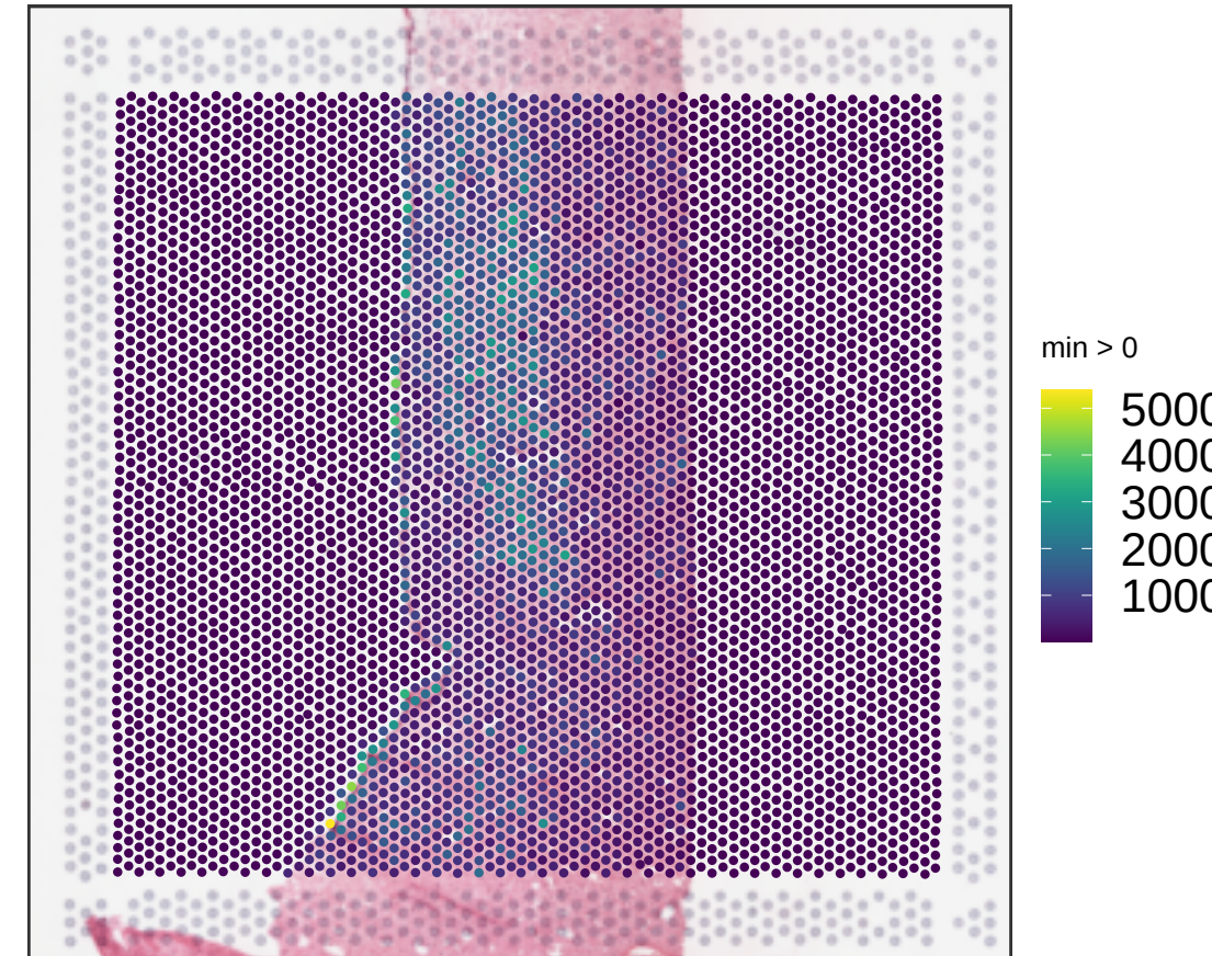
V14F07-340_C1 sum_gene
