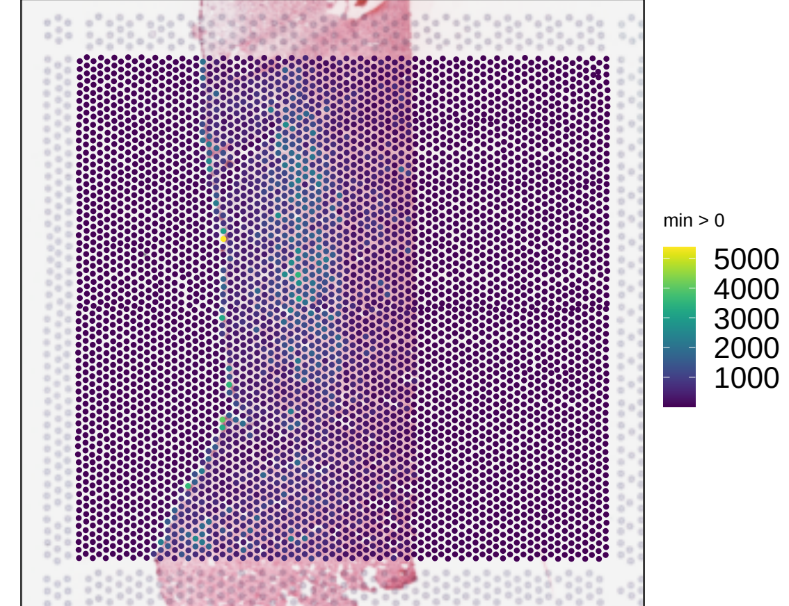
V14F07-340_D1 sum_gene
