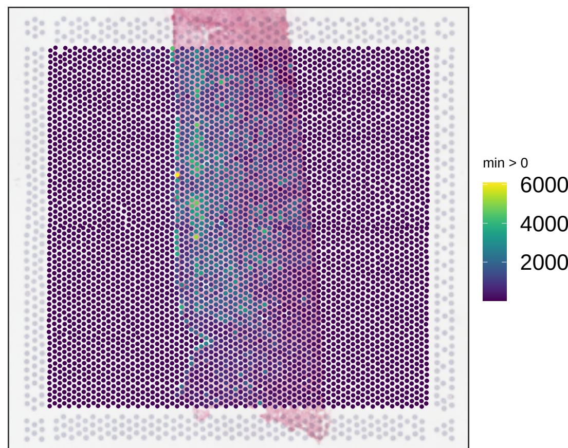
V14F07-340_B1 sum_gene
