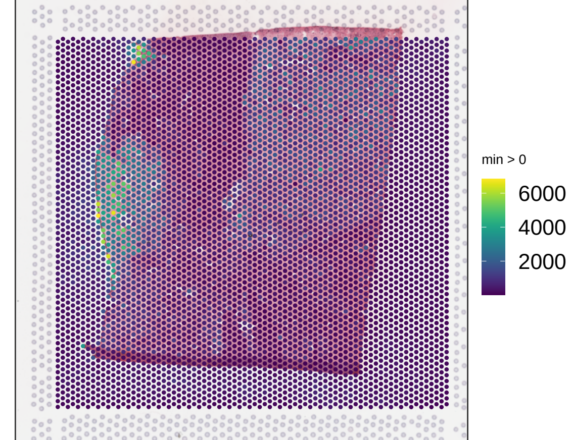
V13B23-285_D1 sum_gene
