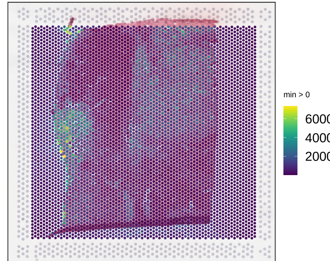
V13B23-285_C1 sum_gene
