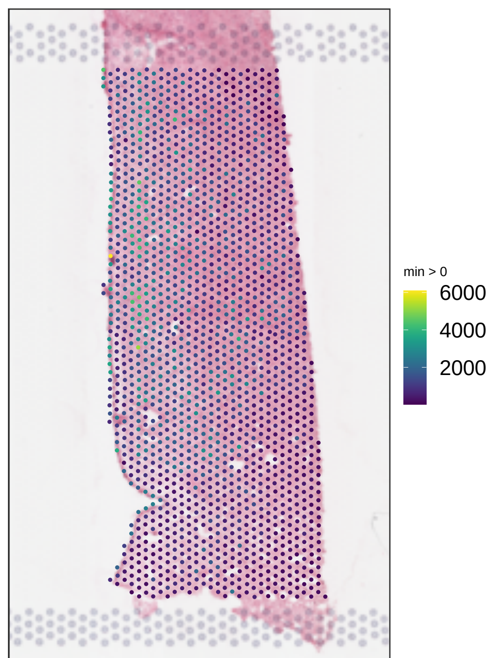
V14F07-340_B1 sum_gene
