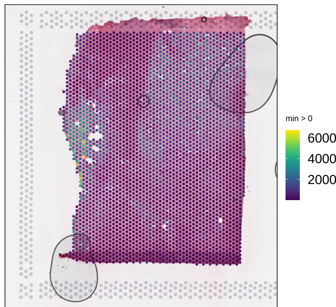
V13B23-285_B1 sum_gene
