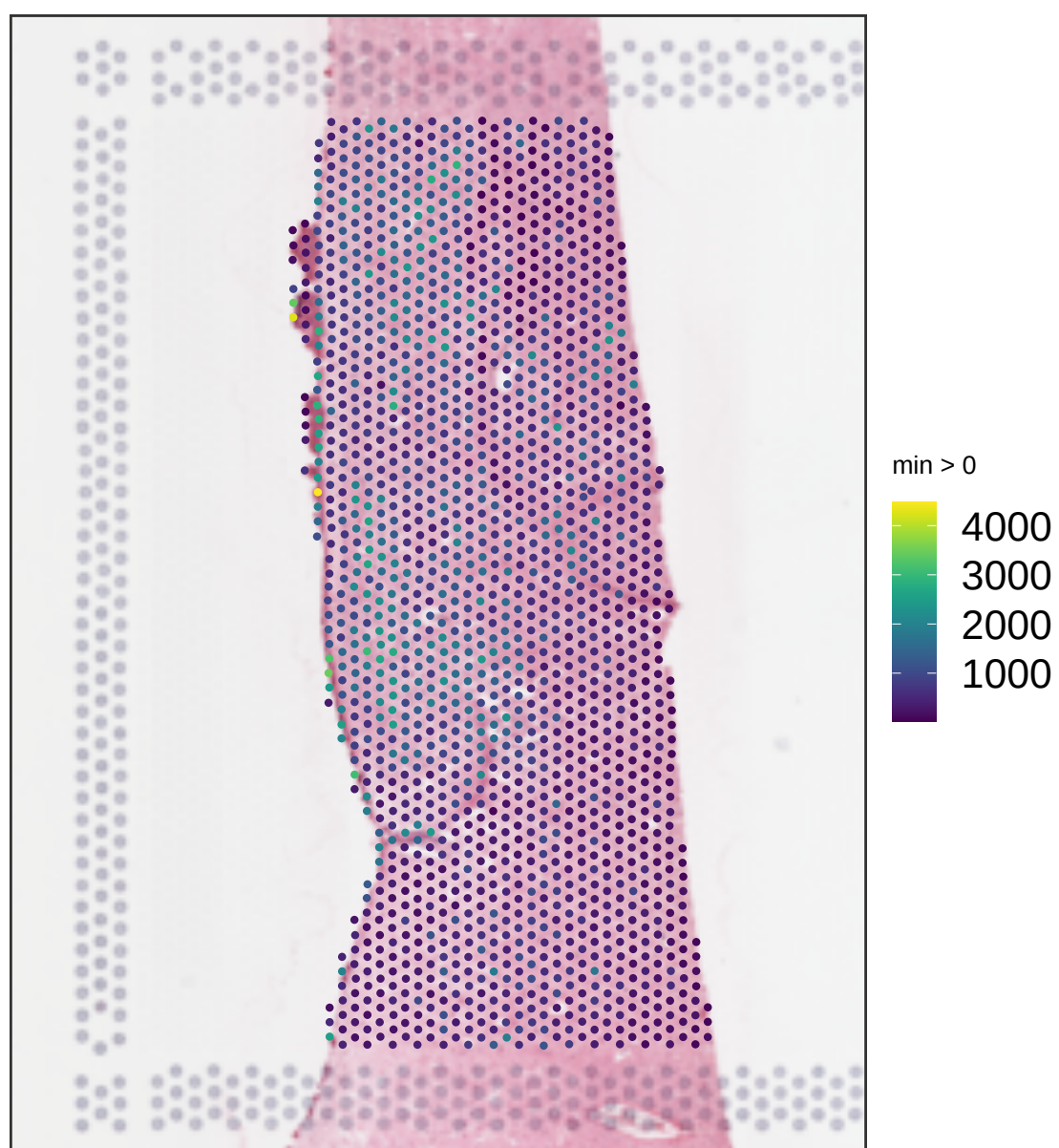
V14F07-340_A1 sum_gene
