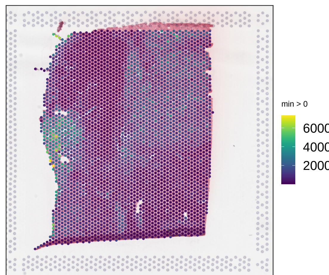
V13B23-285_C1 sum_gene
