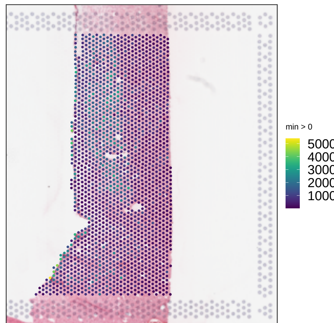
V14F07-340_C1 sum_gene
