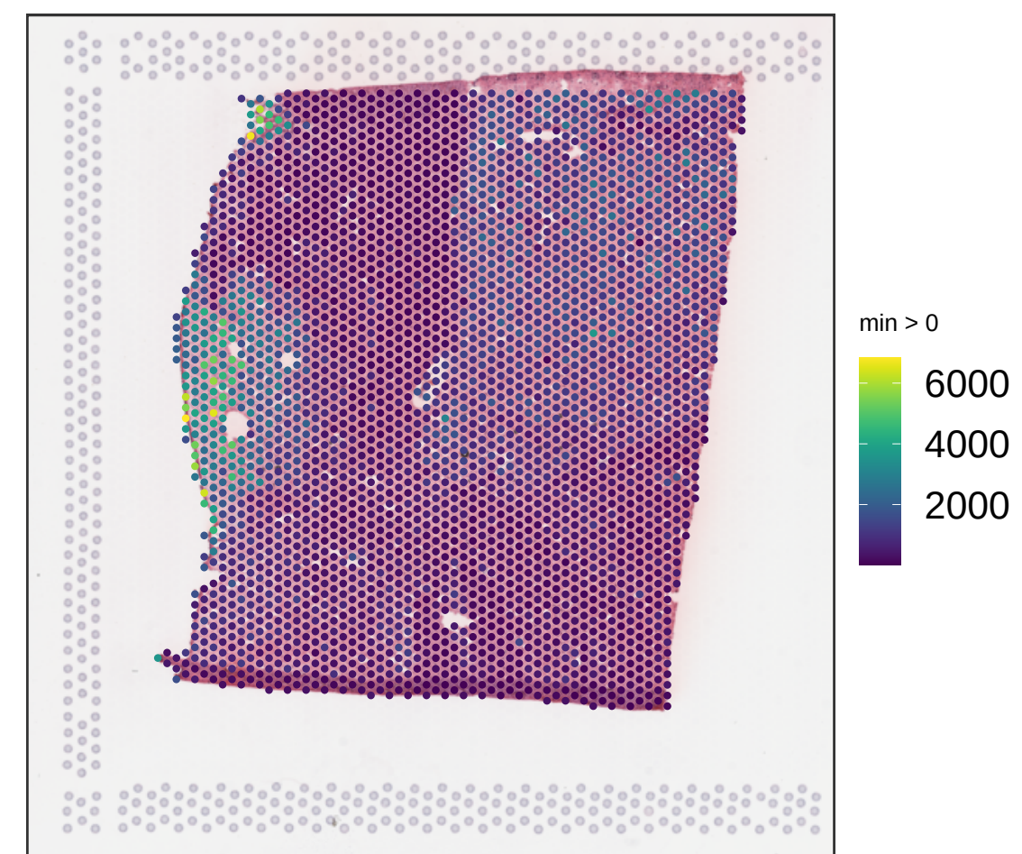
V13B23-285_D1 sum_gene
