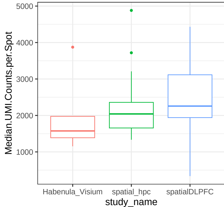
Median.UMI.Counts.per.Spot
