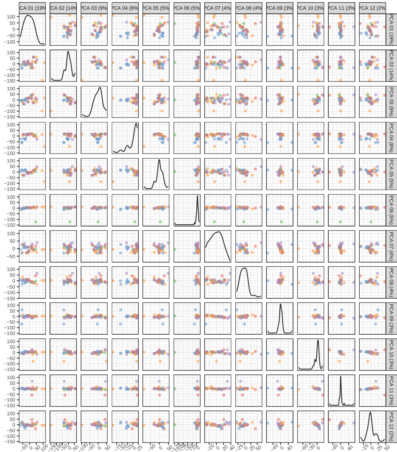
PCA of pseudobulk data with BS k=8
