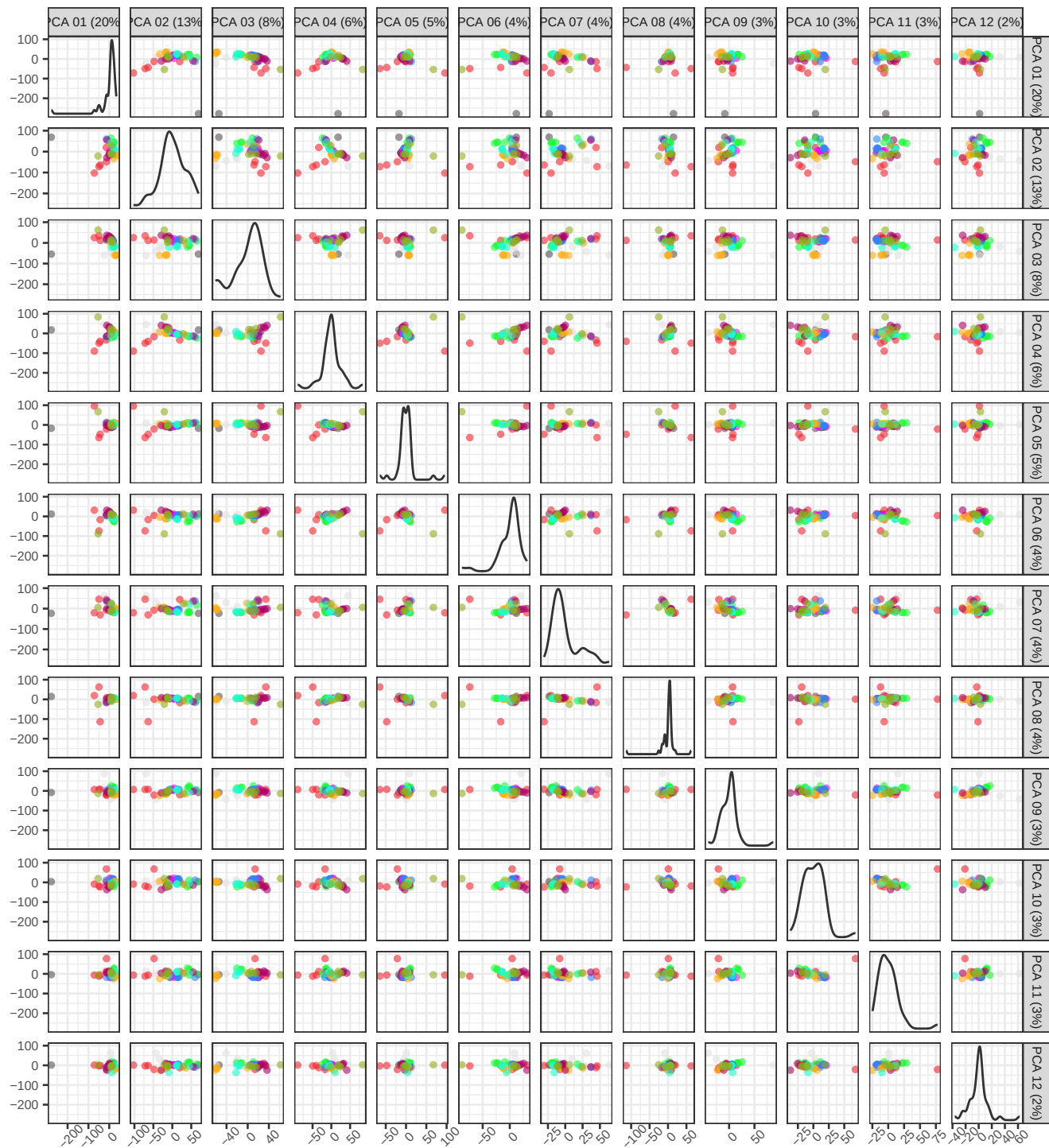
PCA of pseudobulk data with BS k=10
