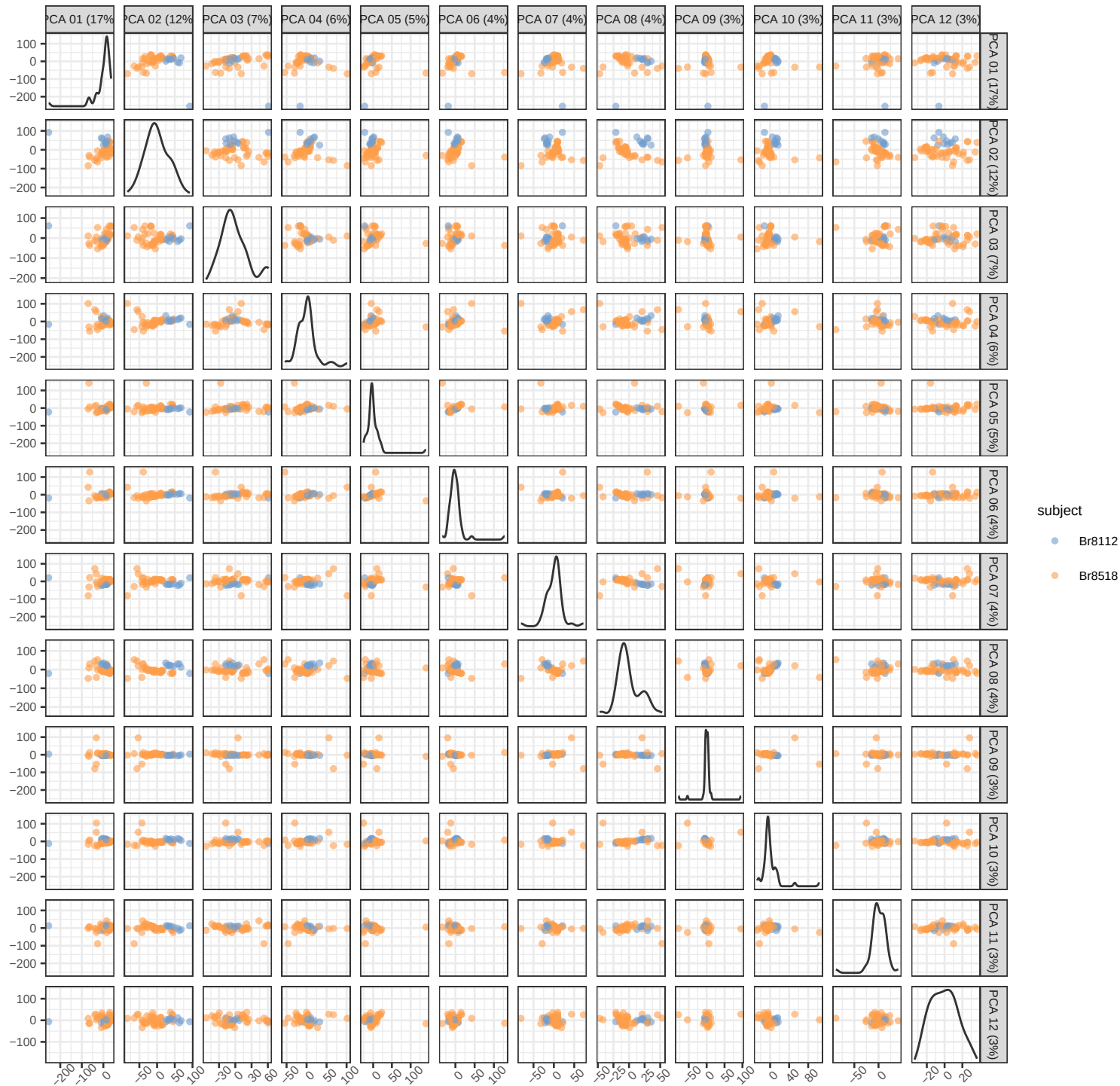
PCA of pseudobulk data with BS k=11
