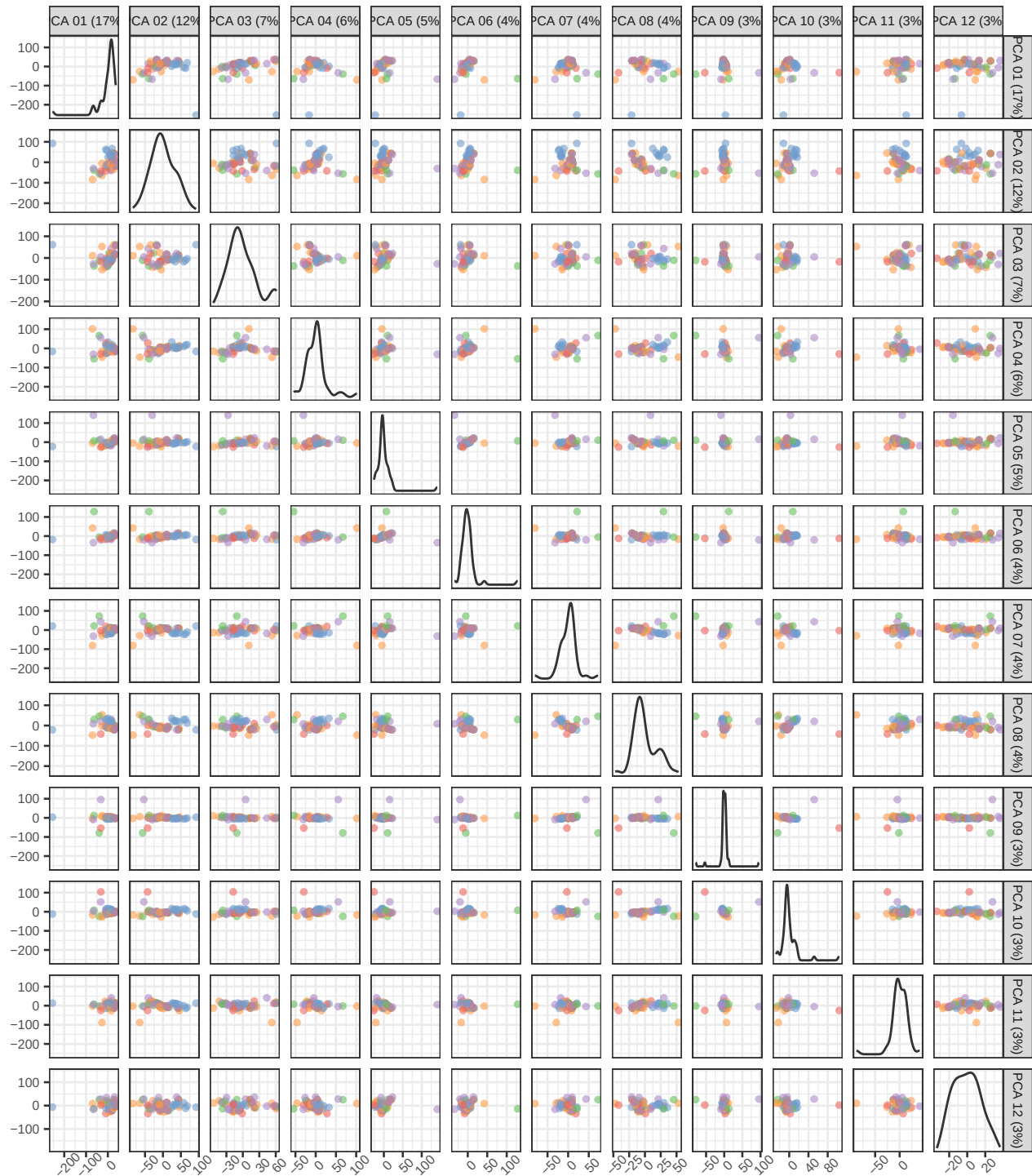
PCA of pseudobulk data with BS k=11
