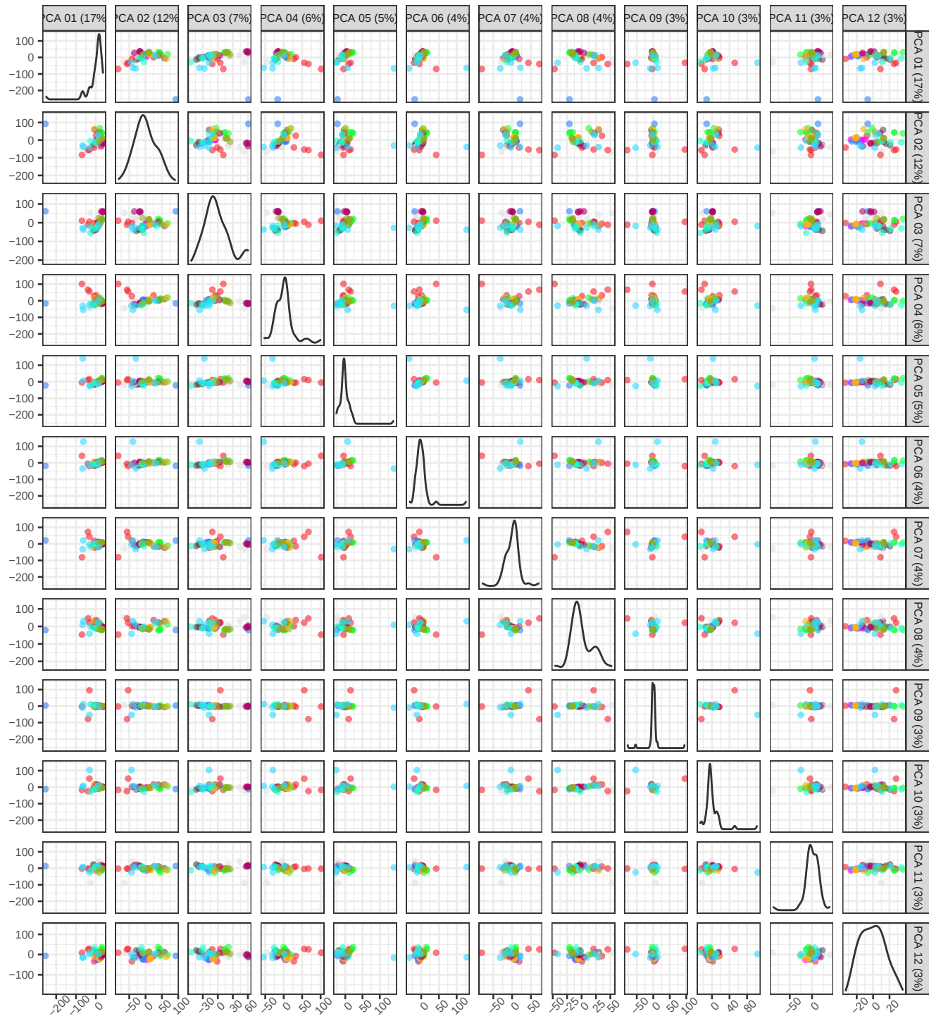
PCA of pseudobulk data with BS k=11
