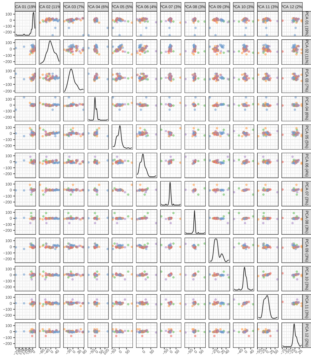
PCA of pseudobulk data with BS k=12
