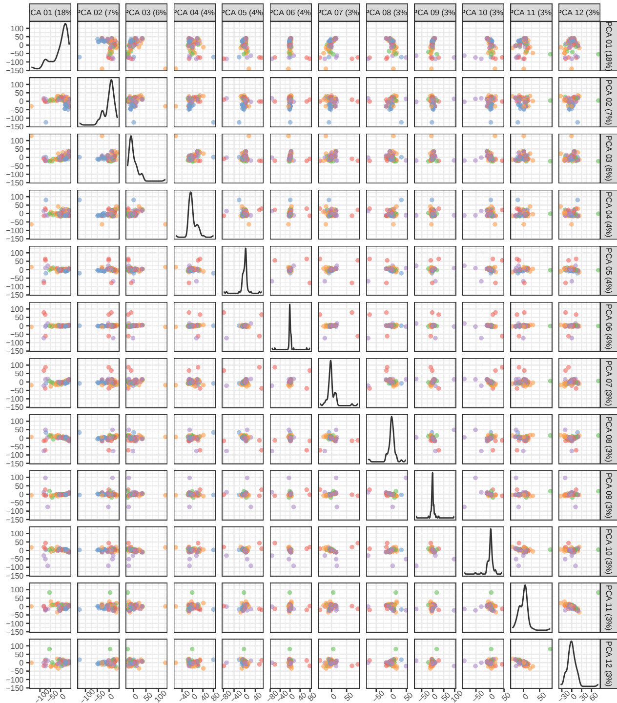
PCA of pseudobulk data with BS k=15
