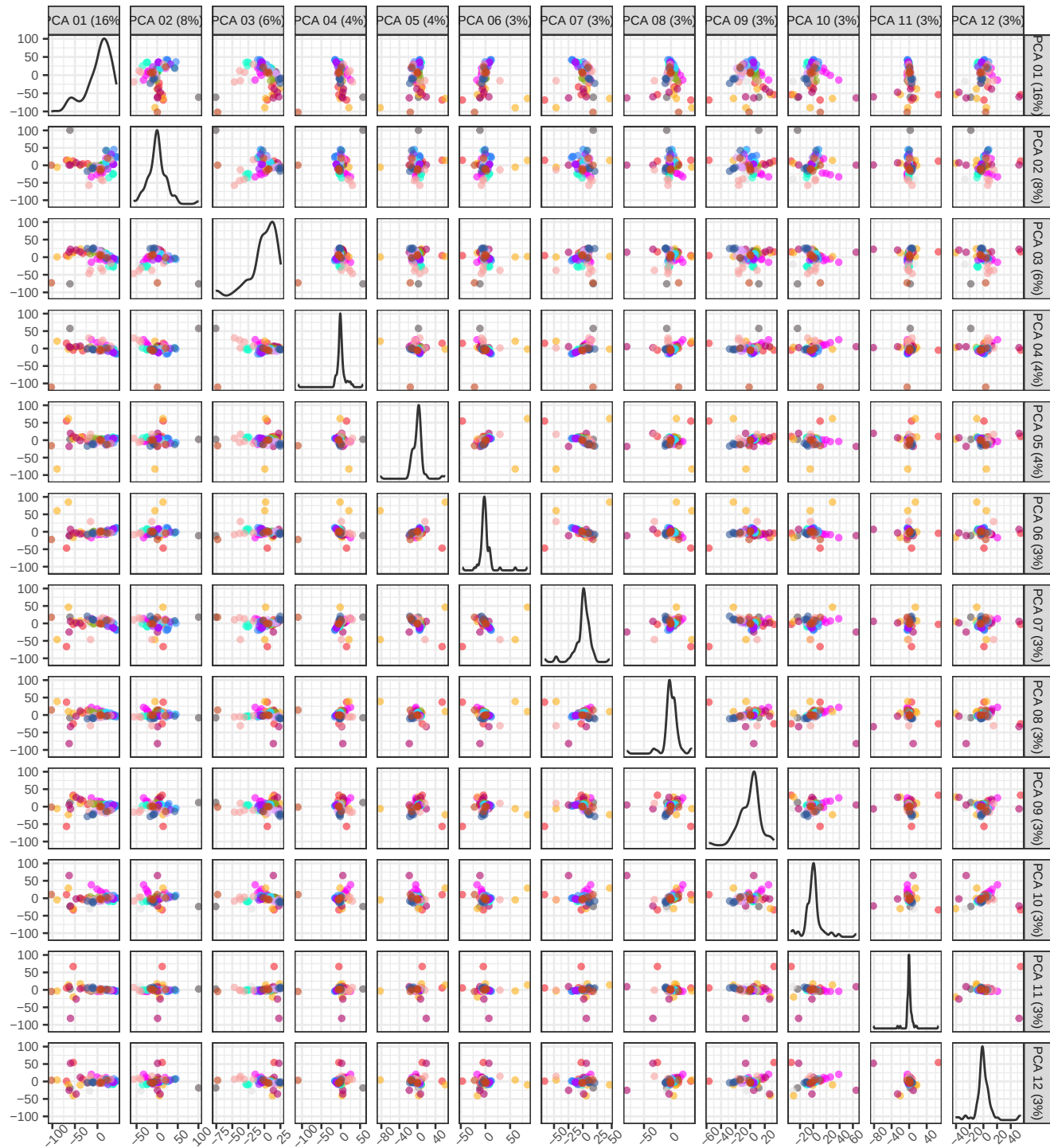
PCA of pseudobulk data with BS k=16
