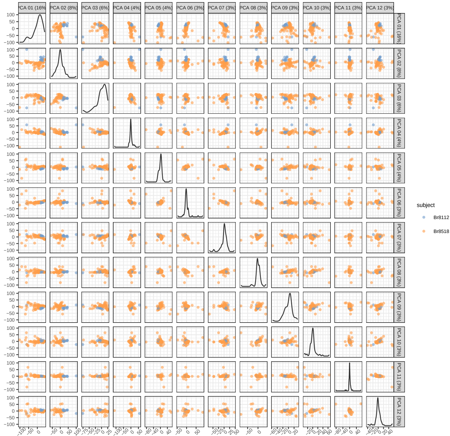
PCA of pseudobulk data with BS k=16
